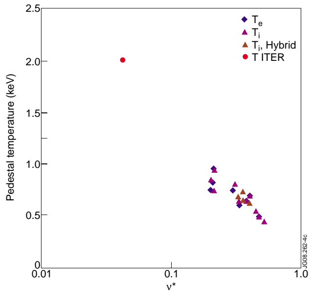
Figure 4: Pedestal temperature as a function of collisionality for radiative type-III ELMy H-modes at JET.
