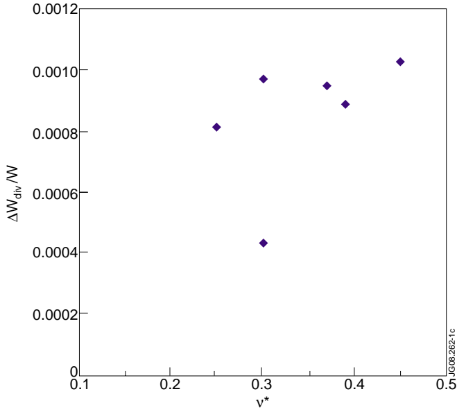
Figure 1: \delta W_{div}/W as a function of collisionality as derived from IR thermography for 2.5MA/2.0T type-III ELMy H-modes.
