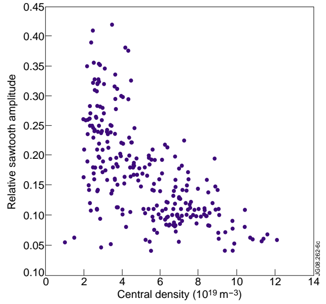
Figure 6: Relative sawtooth amplitude versus central density for JET NBI heated plasmas.
