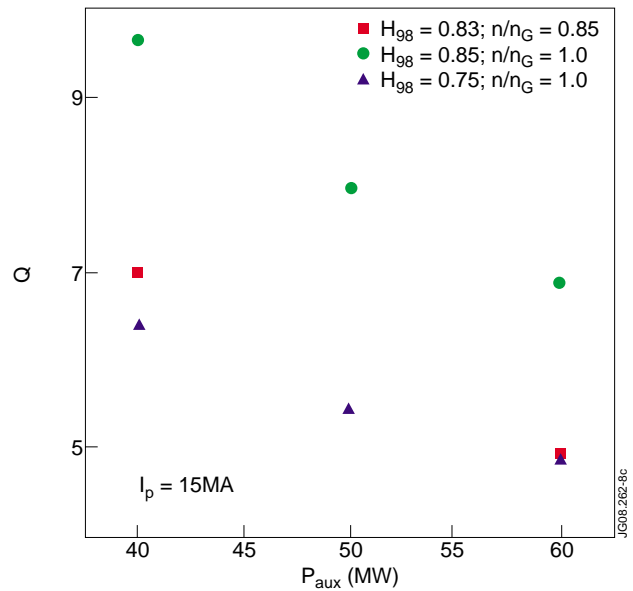
Figure 8: Fusion amplification factor Q versus the auxiliary heating power for the ITER 15MA scenario for radiative scenarios.
