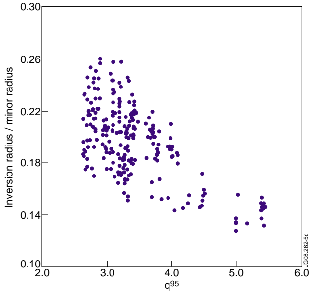
Figure 5: Sawtooth inversion radius normalized to minor radius versus q_{95} for JET NBI heated plasmas.
