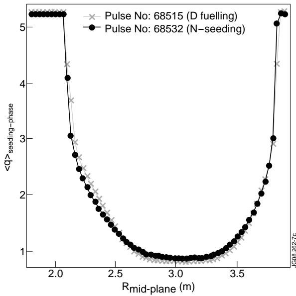
Figure 7: Time average of q -profiles measured by the MSE system during the seeded phase t=[8-11s] for the pulse with D fuelling with type-I ELMs (crosses) and D+N fuelling with type-III ELMs (circles).
