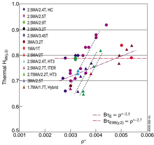
Figure 3: H_{98(y,2)} as a function of normalized gyro radius for radiative type-III ELMy H-modes at JET.
