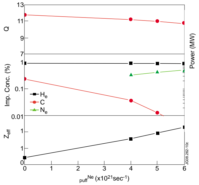
Figure 10: Fusion amplification factor Q , impurity concentration in the core plasma and Z_{\text{eff}} versus the neon gas fuelling rate for ITER 17MA scenario.
