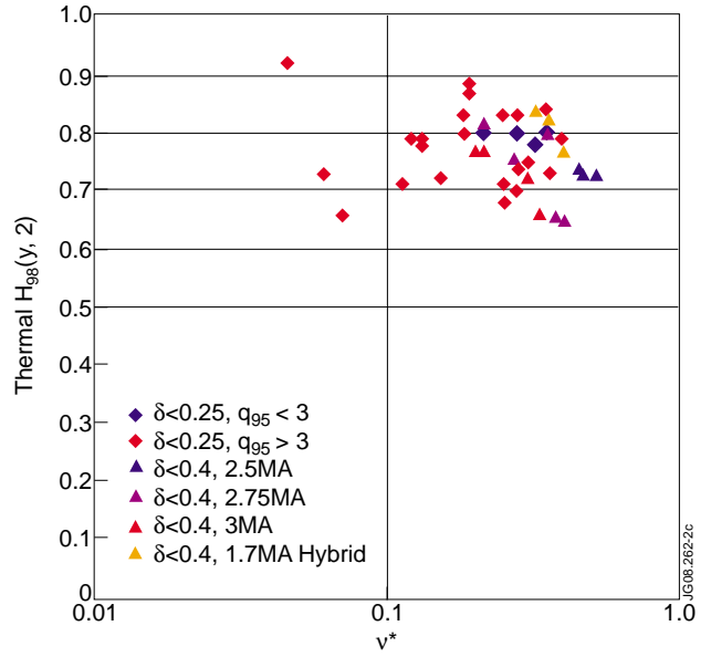
Figure 2: H_{98(y,2)} as a function of collisionality for radiative type-III ELMy H-modes at JET.
