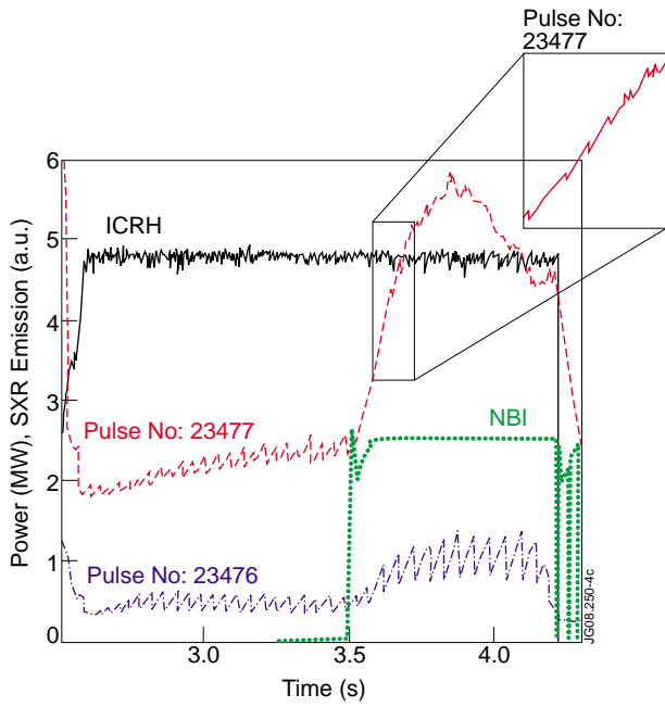
Figure 3: ASDEX Upgrade Pulse No's: 23476 and 23477 show a change in sawtooth behaviour when the NBI is injected near or well outside the q = 1 surface respectively.
