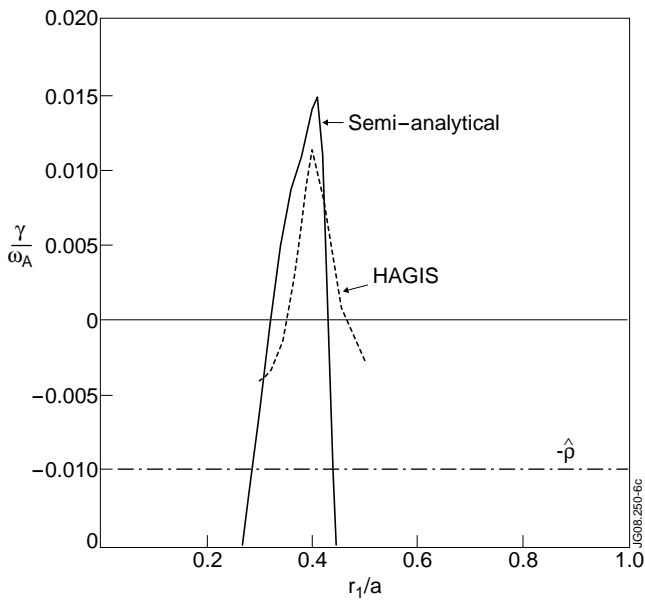
Figure 5: The fast ion growth rate as a function of r_1 . Analytic calculations have been compared with drift-kinetic HAGIS calculations.
