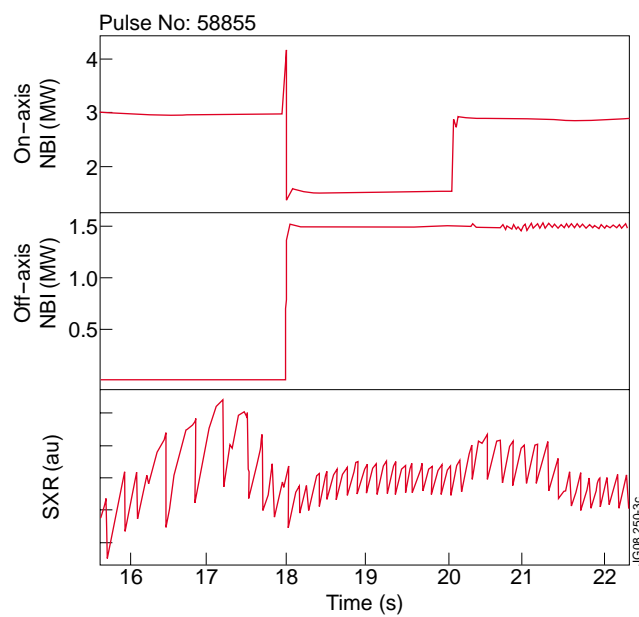
Figure 2: Sawtooth destabilisation from the application of off-axis NBI in JET Pulse No: 58855.
