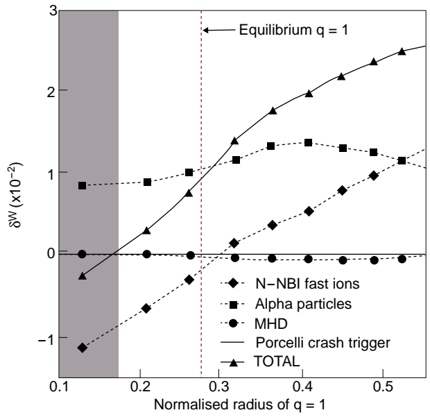
Figure 4: \delta W due to energetic ions in ITER off-axis N-NBI heated plasmas as a function of r_1 . When r_1 is sufficiently core localised the off-axis N-NBI can destabilise the kink mode.
