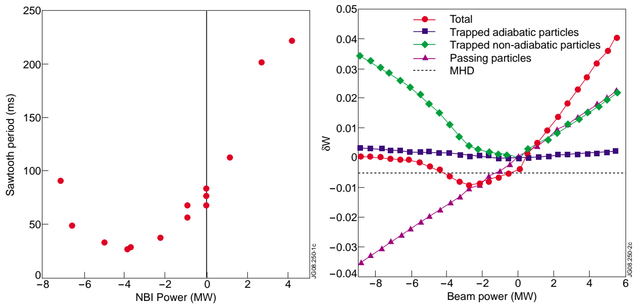
Figure 1: The sawtooth period in JET NBI-heated plasmas compared to the stability of the n = 1 internal kink mode.
