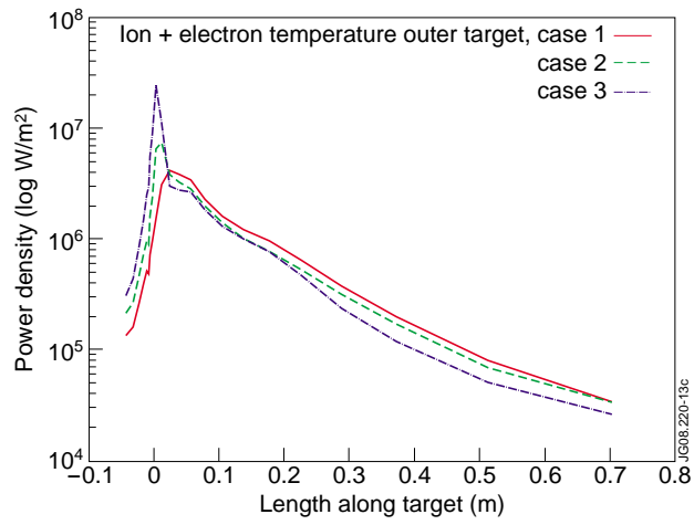
Figure 13: Total power density onto outer target (red- “L-mode”, green- intermediate quality ETB, blue- good quality ETB).
