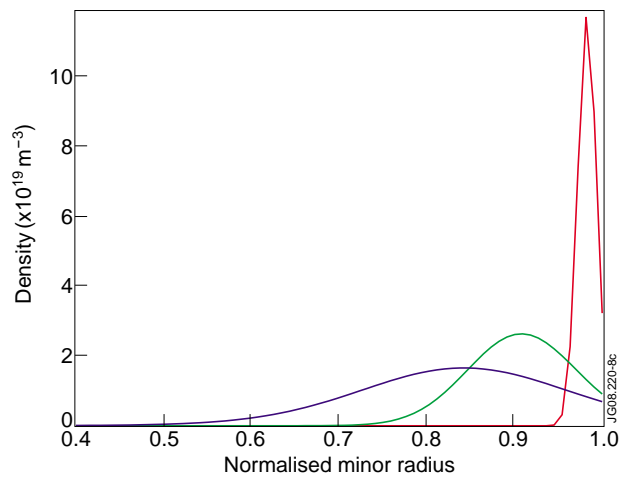
Figure 8: Source profiles for the last injected pellet in 10^{19} \text{ m}^{-3} , samecolour code as for Figure 6.
