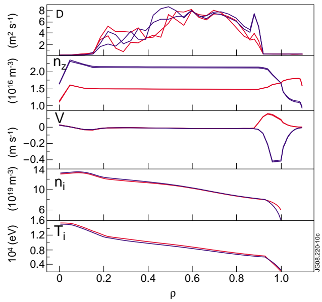
Figure 10. Radial distribution of effective Ar diffusivity: D , (solid- full description, chain line- bundled with 9 super states, red - high edge density, blue - low edge density); total A_r density: n_{Ar} ; effective neo-classical pinch velocity for A_r : V_{Ar} ; main ion density: n_i and ion temperature: T_i .
