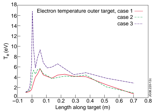
Figure 12: Electron temperature on outer target (red- "L-mode", green- intermediate quality ETB, blue- good quality ETB).
