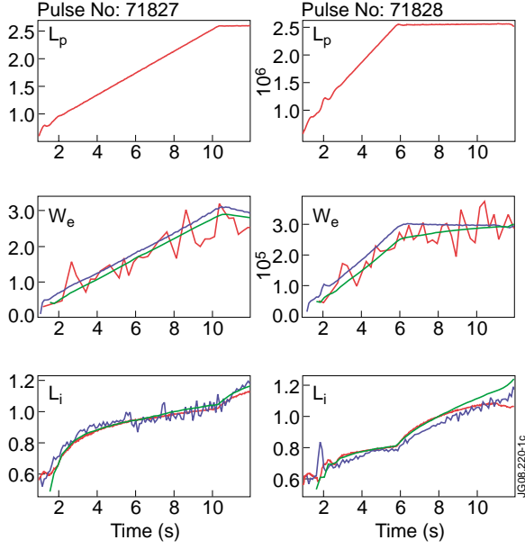
Figure 1: Time evolution of current (top), electron energy content (middle) and internal inductance (bottom): red-exp, blue-CRONOS, green-JETTO.
