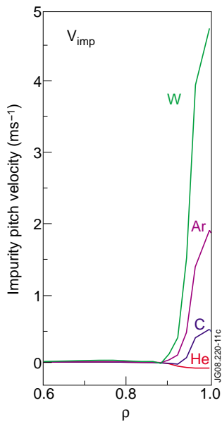
Figure 11: Neo-classical radial pinch velocity for He (red), C (blue), A_r (magenta) and W (green).
