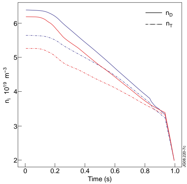
Figure 7: Deuterium density- solid (blue: 100% drift, red: 0% drift), Tritium density- dotted (blue: 100% drift, red: 0% drift).
