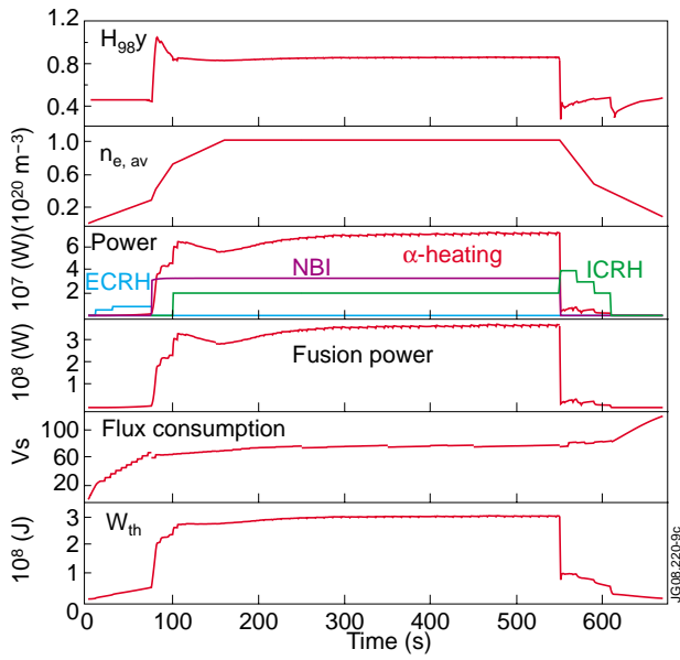
Figure 9: Time traces for predictive modelling of ITER Scenario 2.
