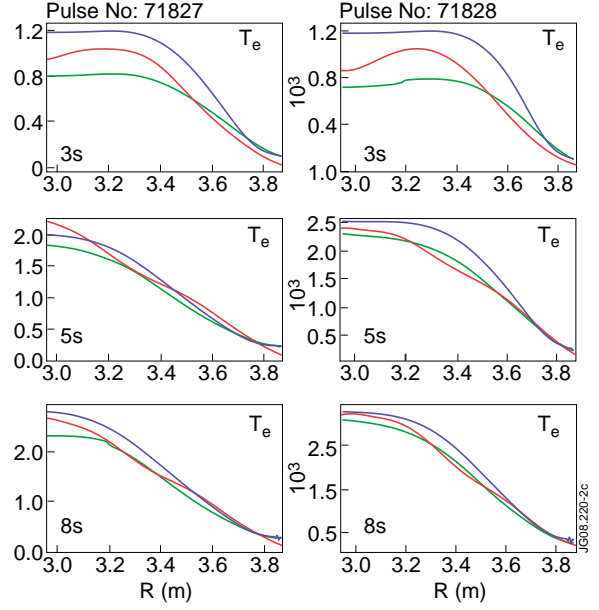
Figure 2: Electron temperature profiles at t=2, 5 and 8 sec: red-exp, blue-CRONOS, and green- JETTO.
