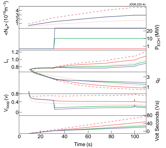
Figure 4: Effect of varying input power and density during ITER I_p ramp-up. The reference simulation (full red lines) has \langle n_e \rangle = 0.25 * n_G , without additional input power. Shown are simulations with 10 and 20MW of ECRH power at mid-radius starting at 30s, at the same density (green and blue, respectively). Also shown are simulations with \langle n_e \rangle = 0.15 and 0.4 * n_G without additional input power (dashed, dotted red lines, respectively). The panels from top to bottom give \langle n_e \rangle , P_{ECHR} , I_p , q(0) , V_{loop} and the flux consumption.
