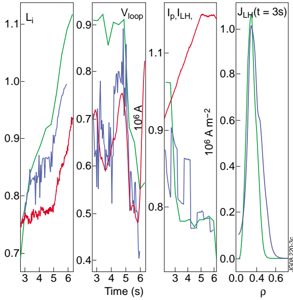
Figure 3: JET Pulse No: 72823, time traces of (from left to right): internal inductance, loop voltage, current and LH current profile (red-experiment, blue- CRONOS and green- JETTO).
