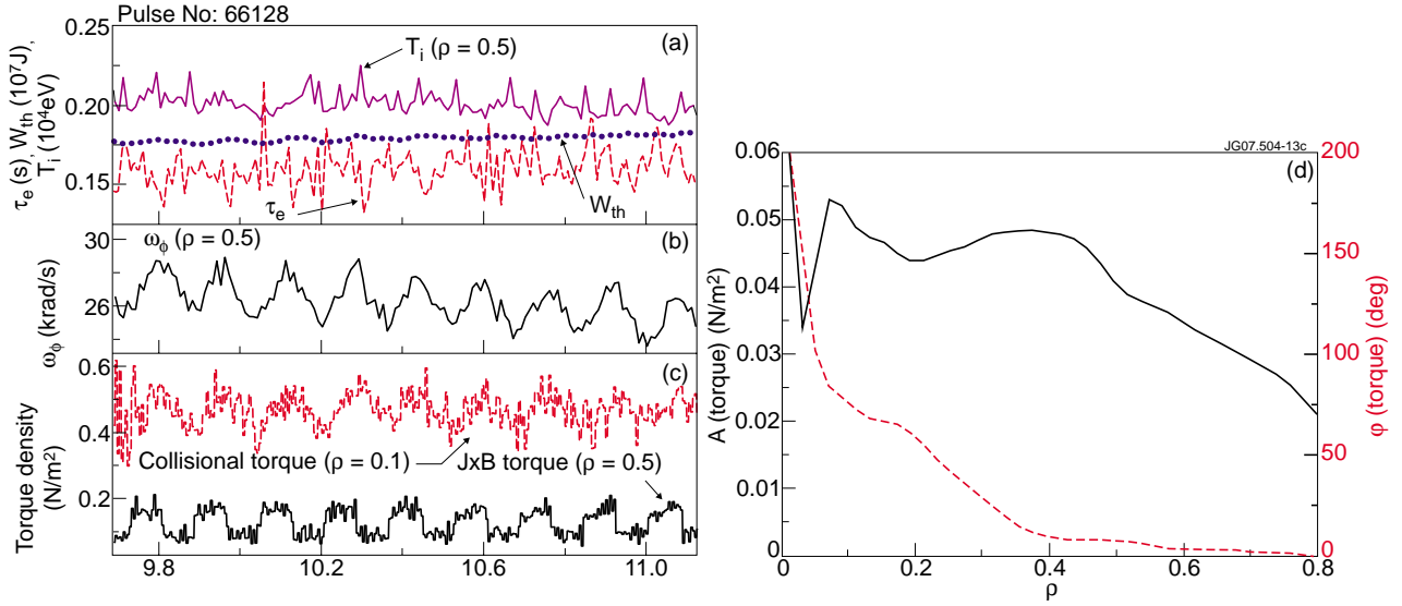
Figure 2. Time traces of (a) T_i , stored thermal energy W_{th} and confinement time \tau_e , (b) toroidal angular frequency \omega_\phi , (c) two components of the torque density for JET Pulse No. 66128. (d) Amplitude (solid black) and phase (dashed red) of the modulated calculated total torque.
