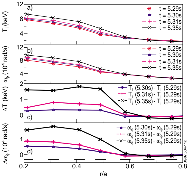
Figure 6. (a) T_i , (b) \omega_\phi , (c) \Delta T_i and (d) \Delta \omega_\phi profiles for JET Pulse No: 69670 during the radial expansion of the ITB. The horizontal lines shown in frame (d) indicate the radial widths of the CXRS measurements points.
