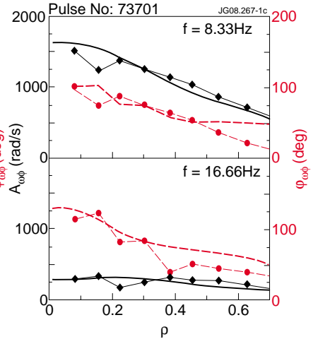
Figure 5(c): Experimental amplitude (black solid with squares) and phase (red dashed with squares) and simulated amplitudes A_{\omega,\phi} (black solid) and phases \phi_{\omega,\phi} (red dashed) of modulated \omega_\phi with P_r \approx 1 and v_{pinch} as in figure 4(d) for 1 st harmonic (upper frame) and 2 nd harmonic (lower frame).
