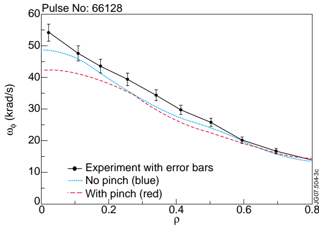
Figure 3. The simulated steady-state \omega_\phi with the two options (i) with P_r = 0.25 and v_{pinch} = 0 and frame (b) (dotted blue) and (ii) with P_r \approx 1 and v_{pinch} taken from figure (d) (dashed red) compared with the experimental \omega_\phi (solid black) with error bars.
