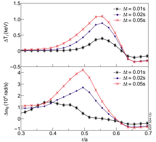
Figure 7. As in figure 6, but for simulated (a) \Delta T_i and (b) \Delta \omega_\phi profiles with a model of v_{pinch} \approx -15 \text{ m/s} and P_r = 1.0 .
