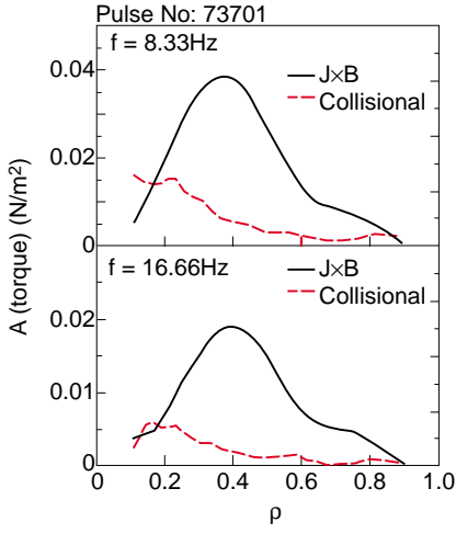
Figure 5(a): Different components of the modulated torque for JET Pulse No: 73701 for 1 st harmonic (upper frame) and 2 nd harmonic (lower frame).
