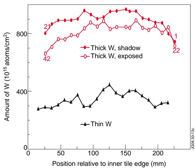
Figure 2: RBS data showing the W levels on tile 5 stripes and masks.
