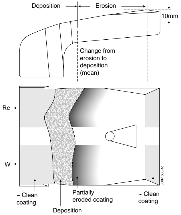
Figure 4: Schematic of IWGL tile 7Z12L after exposure, and the distances from the leading edge of the tile.
