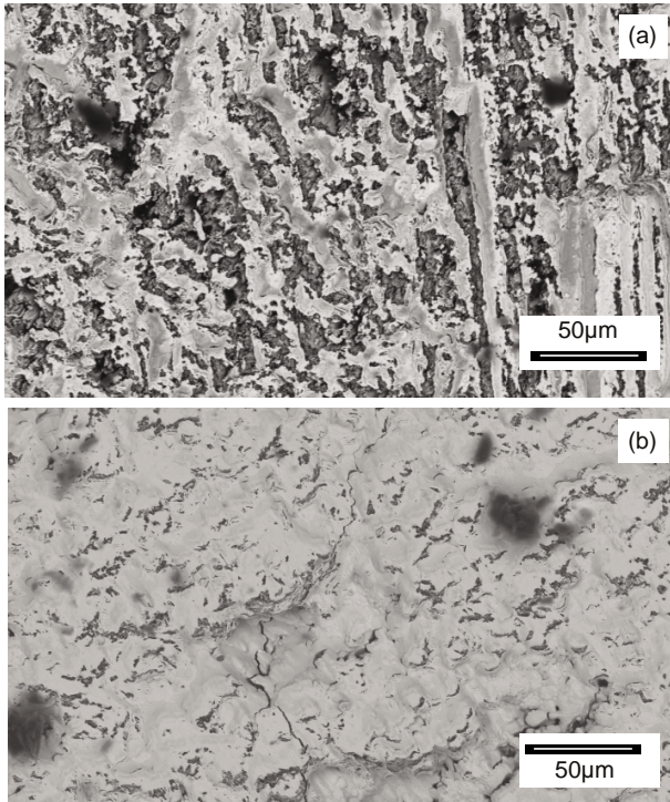
Figure 3: SEM photographs from tile 5 (a) on the plasma-exposed part of the thicker W stripe (b) on the thinner stripe
