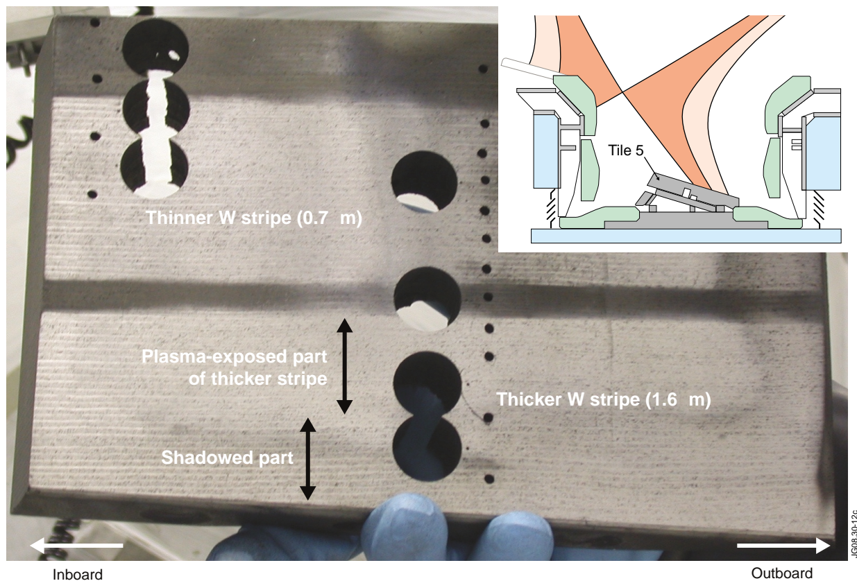
Figure 1: Photograph of JET divertor tile 5, coated with two stripes of W, after exposure and removal of core samples for SEM analysis. Inset shows the divertor configuration.
