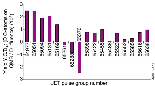
Figure 4: yield YC/D^+ of carbon atom deposited/eroded on the quartz depending on D^+ fluence into a toroidal section of 1cm length of the inner divertor.
