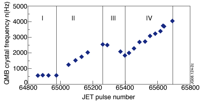
Figure 2: carbon layer formation on QMB in the PFR of JET; change over from deposition (II) to erosion (III) and back to deposition (IV).
