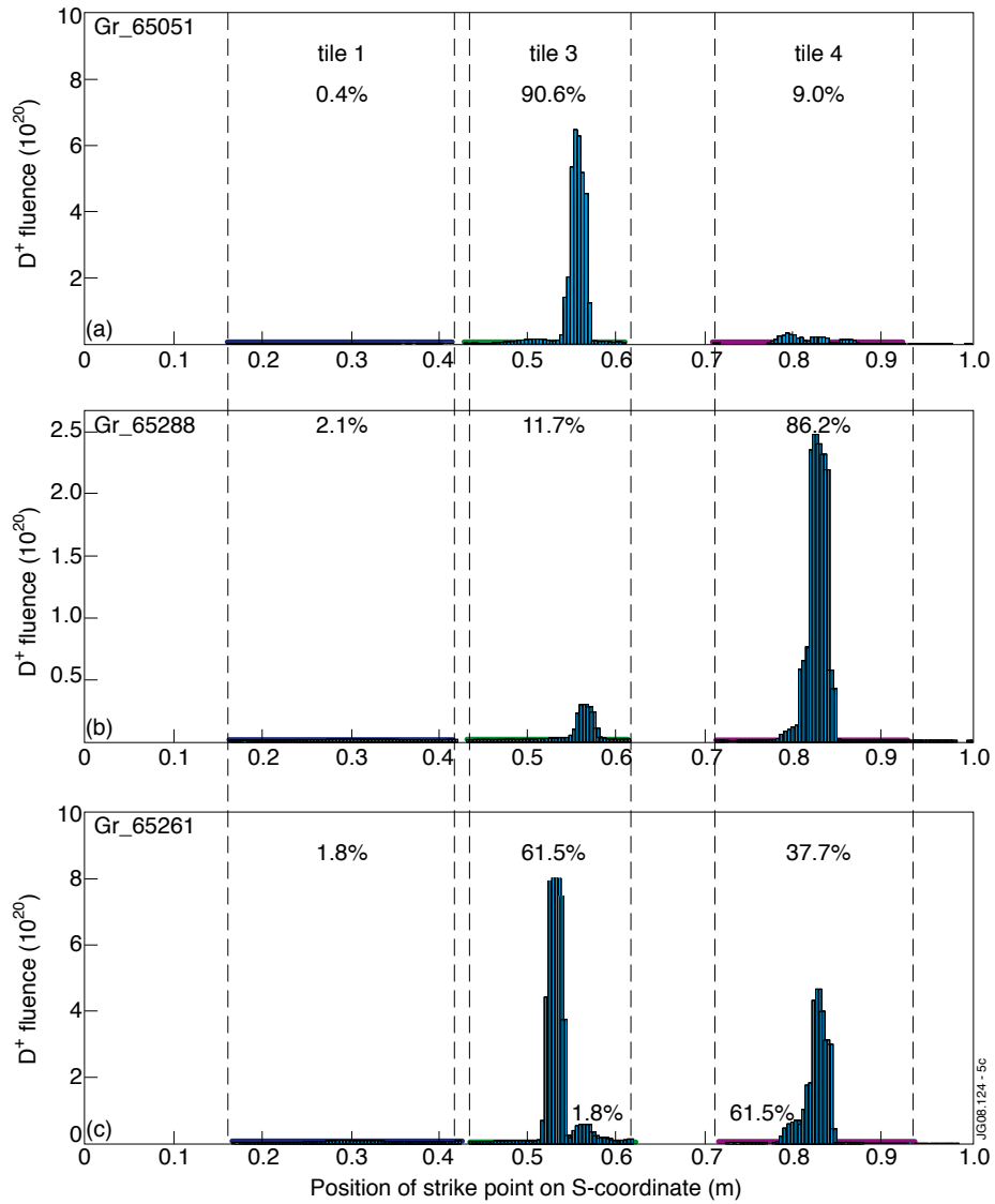
Figure 5: Typical D^+ fluence distribution for to the tiles 1, 3 and 4 in the inner divertor for (a) deposition, (b) erosion and (c) reduced erosion
