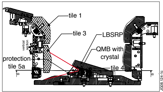
Figure 1: location of QMB in private flux region of the MKII - HD divertor of JET.
