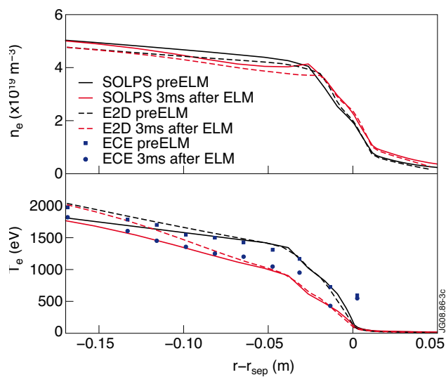
Figure 3: Pre-ELM and ELM upstream profiles for Pulse No: 58569, up: n_e from SOLPS and EDGE2D, down: T_e from SOLPS, EDGE2D and ECE.
