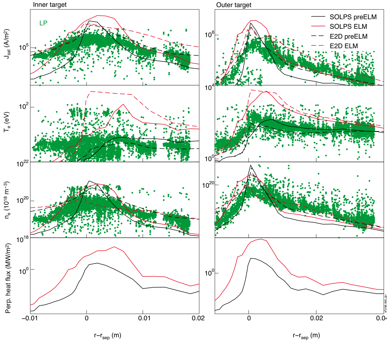
Figure 4: Pre-ELM and ELM target profiles, j_{sat} , T_e , n_e from EDGE2D and SOLPS, Perp.heat fluxes from SOLPS.
