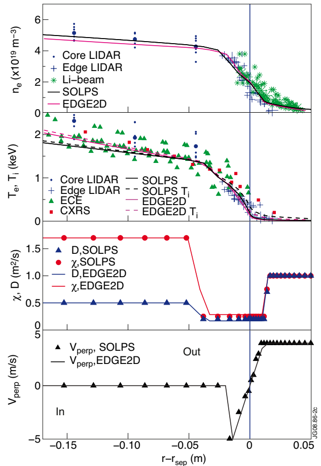
Figure 2: Pre-ELM n_e , T_e , T_i upstream profiles for Pulse No: 58569, Exp. Data, SOLPS and EDGE2D, corresponding radial profiles of D_{\perp} , \chi_{\perp e} , \chi_{\perp i} , v_{\text{perp}} .
