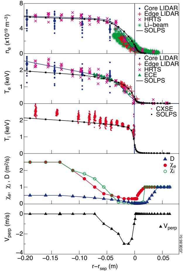
Figure 5: Pre-ELM upstream n_e, T_e, T_i profiles for Pulse No: 70224, Exp. data and SOLPS, corresponding radial profiles of D_{\perp}, \chi_{\perp e}, \chi_{\perp i}, v_{perp} .
