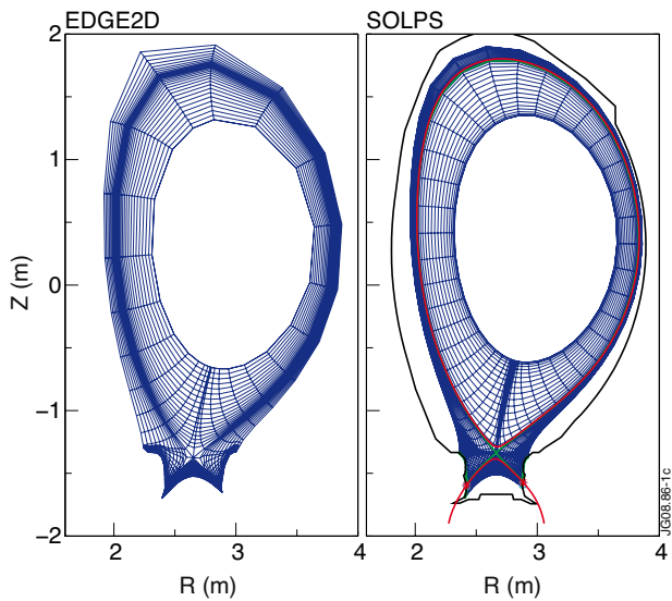
Figure 1: Simulation grids, on the left: EDGE2D, on the right: SOLPS (red line= separatrix from EFIT, green line=SOLPS separatrix).
