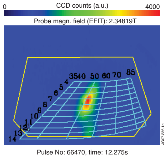
Figure 1: Scintillator plate contour with phasespace grid (gyro radius in cm and pitch angle in degrees) just after sawtooth reconnection event. Prompt losses (lower right) and purely sawtooth induced losses (upper left) 50 ms after crash
