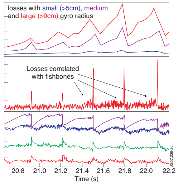
Figure 2: Pulse No: 66486 with repetitive sawtooth activity. Top: CCD camera integral signal over different gyro radii, Middle: Photomultiplier total photon count, Lower: Soft X-ray temperature traces
