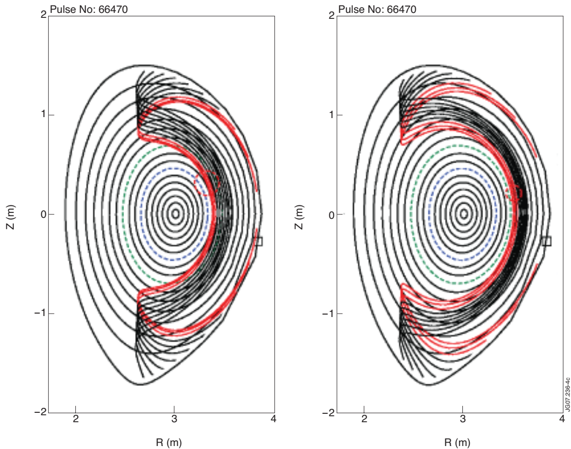
Figure 4: Left: Loss orbits with 12cm, 56^\circ signature at probe detector Right: Loss orbits with 8 cm, 52^\circ signature at probe detector Guiding center orbits which may hit the probe are colored red, the small circle has the size of the gyro radius, the sawtooth inversion radius is blue, the q=1.5 surface green, IC resonance plane aligns with the banana tips in the left. Detector position is indicated by small rectangle (LFS).
