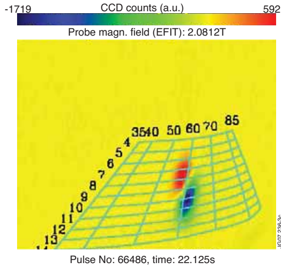
Figure 3: Difference plot at sawtooth time. Red spot indicates losses after sawtooth, blue spot shows maximum before the crash.
