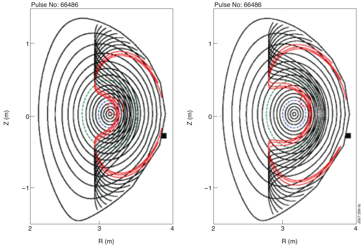
Figure 5: Left: Orbits with (10.5\text{cm}, 60.5^\circ) at detector, guiding centre within sawtooth inversion. Right: Orbits with (8\text{ cm}, 58^\circ) , guiding centre always outside inversion radius, detector position indicated by small black rectangle.
