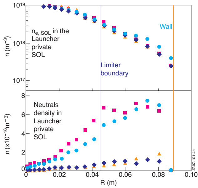
Figure 4: Upper figure: n_{e,SOL} as a function of the heating and puff rates, at the bottom figure there are corresponding neutrals profiles in the OMP. Blue diamonds: 0 heating, 0 puff, magenta rectangulars: 0 heating, puff = 1e22 el/s, yellow triangles: heating = 150 kW, 0 puff, Cyan circles: heating = 150 kW, puff = 1e22 el/s.
