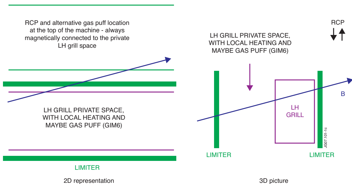
Figure 1. Schematic representation of the 2D and 3D configuration of the LH grill and RCP.
