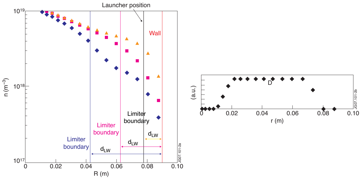
Figure 2: Left figure: Effects of the limiter boundary location. x- axis: distance from separatrix in m. Right figure: Profile “D” of the LH field dissipation (a.u.)” Series 1 (blue diamonds): d_{LW} = 4.75\text{cm} (grill \sim 3\text{cm} behind the limiter), series 2 (magenta rectangles): d_{LW} = 2.75\text{cm} (grill \sim 1\text{cm} behind the limiter), and series 3 (yellow triangles): d_{LW} = 1.25\text{cm} (grill is \sim flush with the limiter).
