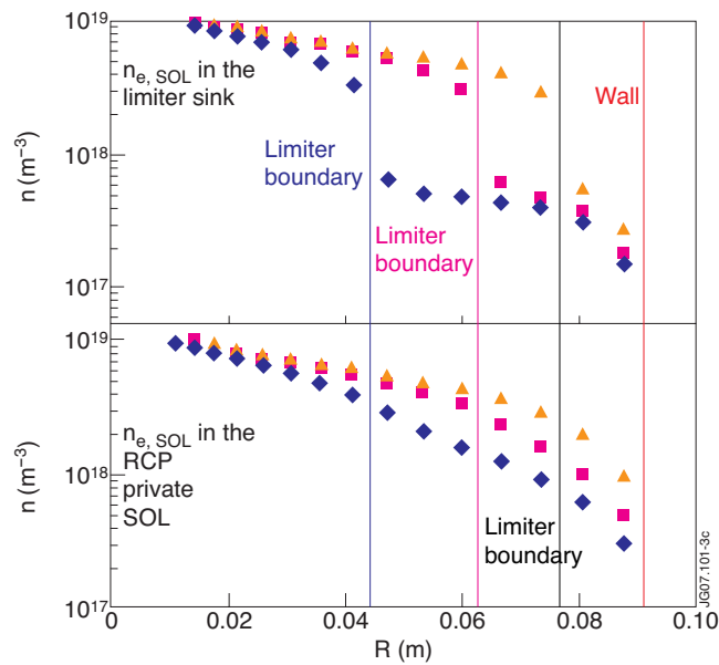
Figure 3: Profiles of n_{e,SOL} near limiters and in the RCP private SOL.
