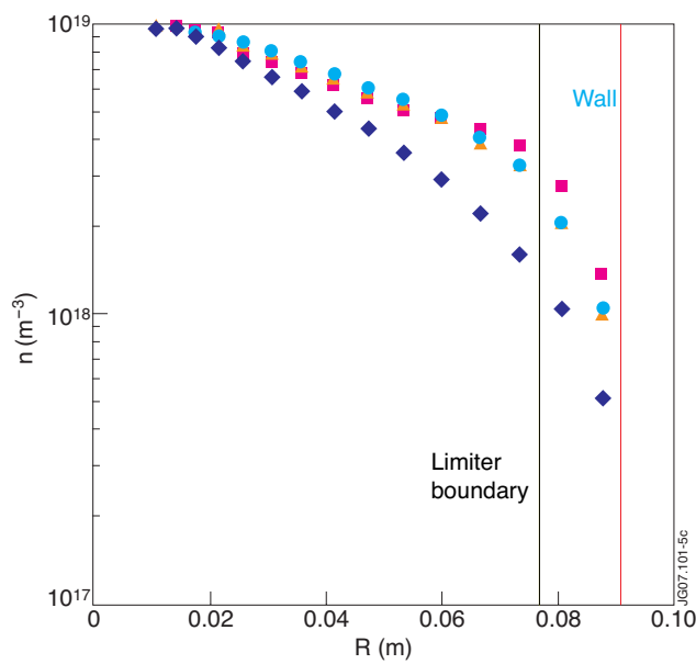
Figure 5: Profile of n_{e,SOL} in the OMP in grill private SOL, as a function of the gas puff location. Blue diamonds: 0 heating, 0 puff, magenta rectangulars: gas puff 1e22 el/s near OMP, yellow triangles: gas puff near RCP, cyan circles: gas puff at the top.
