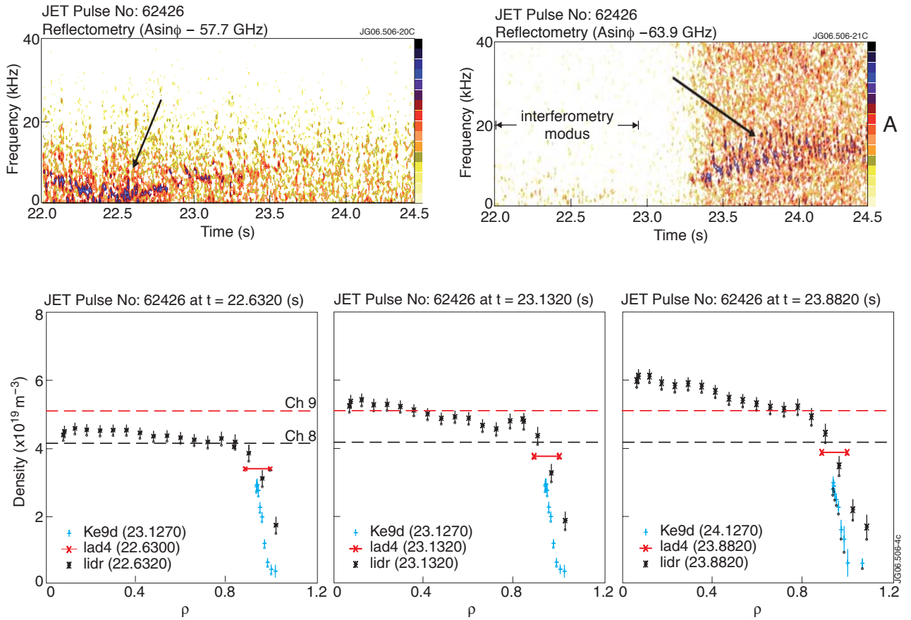
Figure 3: Spectrograms of \text{Asin}\phi -signals for two reflectometer channels with n_{e,\text{cutoff}} = 4.13 \times 10^{19} \text{ m}^{-3} (top left) and 5.07 \times 10^{19} \text{ m}^{-3} (top right) during a density ramp up. The density fluctuations switch channels at t = 23.3 s. A sequence of density profiles for three different times is shown below, together with the respective cut-off positions of reflectometry (horizontal lines), indicating radial locations of spectrogram observations. Until \sim 22.9 s the 63.9 GHz channel is in interferometry modus (reflection at inner wall).
