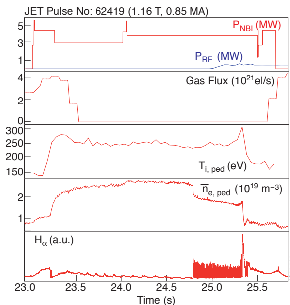
Figure 1: JET Pulse No: 62419.
