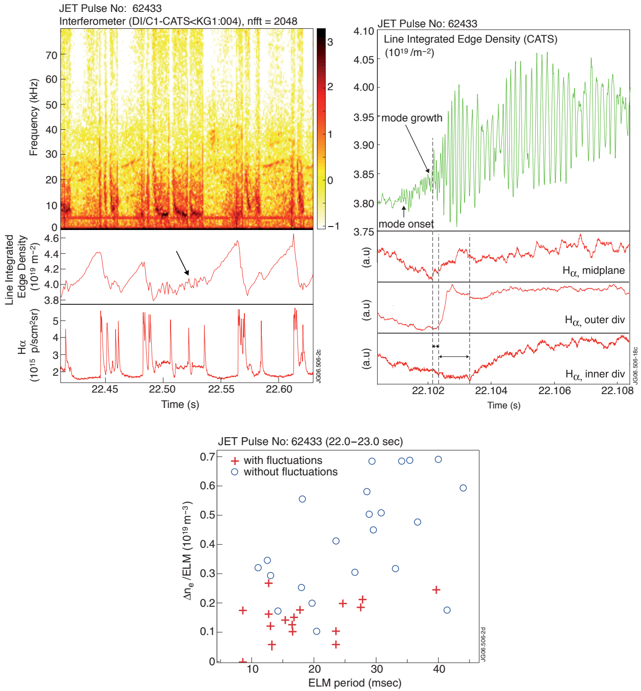
Figure 4: (a) Spectrogram of the edge chord signal of the FIR interferometer, showing isolated phases with density fluctuations between some type-I ELMs. Also shown are the line-integrated edge density and the H emission in the outer divertor. (b) Timings for onset of enhanced emission at various locations (c) comparison of ELM-induced particle losses for ELM periods with and without the density fluctuations
