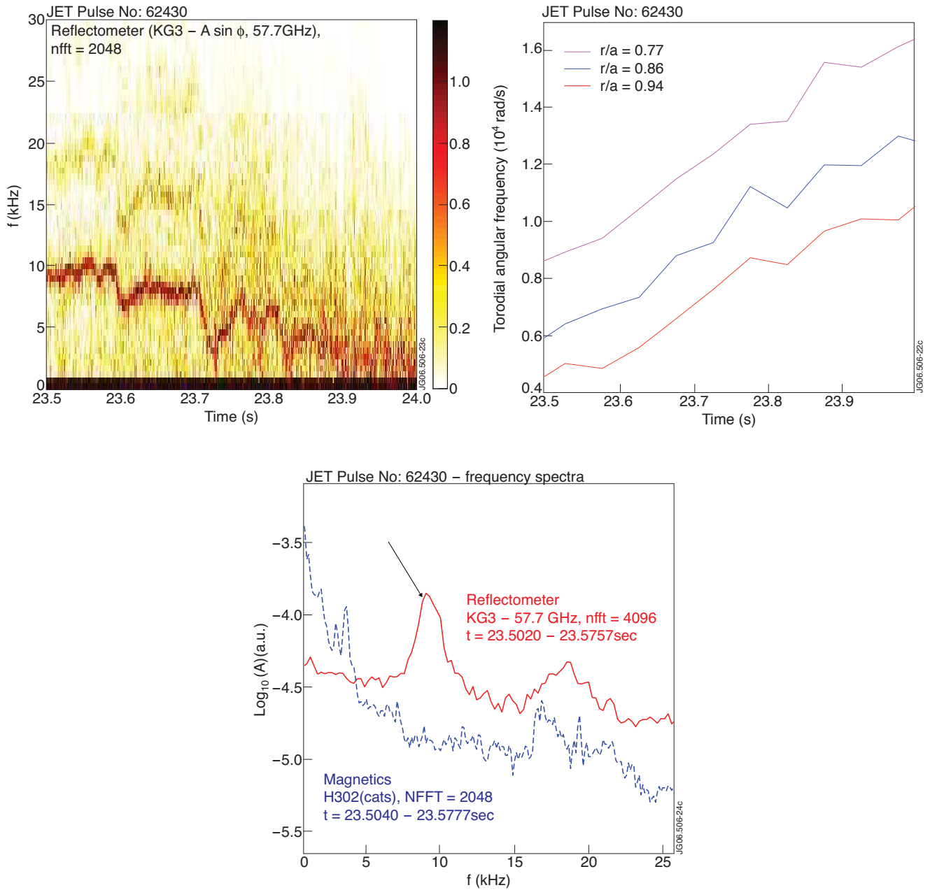
Figure 2: (a) Spectrogram from reflectometry showing narrowbanded density fluctuations, (b) comparison of frequency spectra from reflectometry and fast magnetics. The density fluctuations are not detected on the magnetic fluctuation signal. (c) Time evolution of the edge plasma rotation, obtained by charge exchange recombination spectroscopy.
