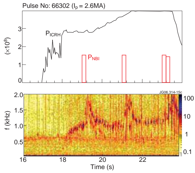
Figure 6: Spectrogram of magnetic pick up signal showing frequency of sawtooth precursors that increase with P_{ICRF} .
