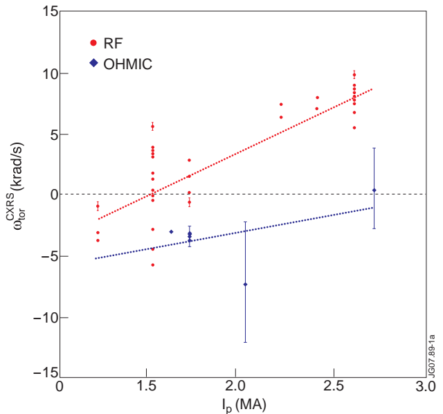
Figure 5: Central Toroidal Angular Frequency from CXRS measurements versus I_p .
