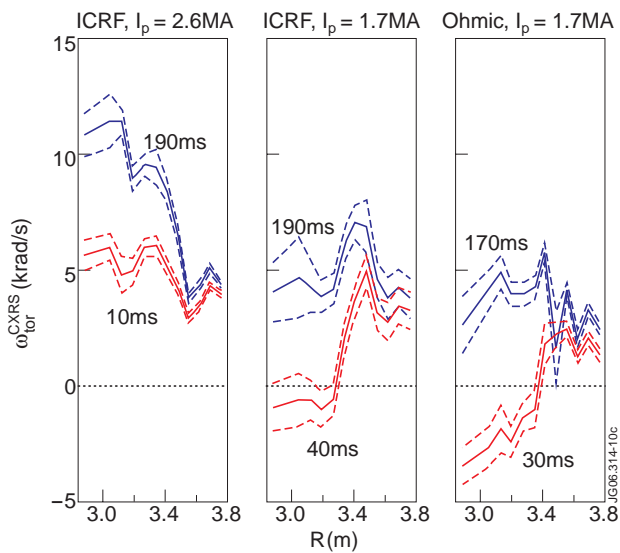
Figure 4: CXRS Toroidal Angular Frequency Profiles for similar discharges: (a) I_p = 2.6MA with ICRH (see fig. 3), (b) I_p = 1.7MA with identical ICRH (c) reference Ohmic plasma with NBI blips but no ICRH. The 1st reliable profile is shown in red and a profile at the end of the blip is shown in blue. The times are from the start of the blip.
