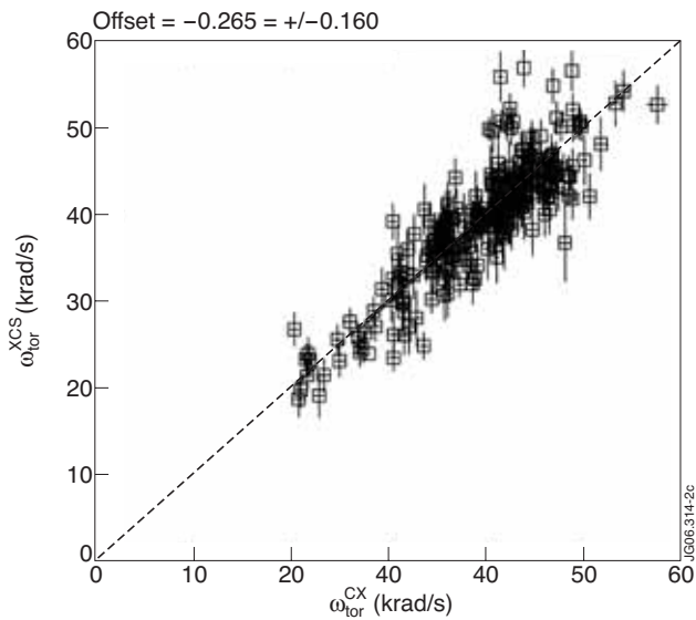
Figure.2 - Comparison of measurements of toroidal angular frequency of C^{+6} and Ni^{+26} at the same radius ( Ni^{+26} \langle R \rangle = 3.2-3.8m. ).
