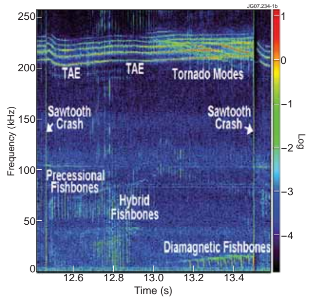
Figure 1(a): Electron temperature, ICRH power, central plasma density and safety factor on axis for a typical monster sawtooth in this scenario (Pulse No: 66378). The different monster sawtooth phases are separated by red lines. Figure 1(b): Spectrogram of MHD activity for the same period of time.
