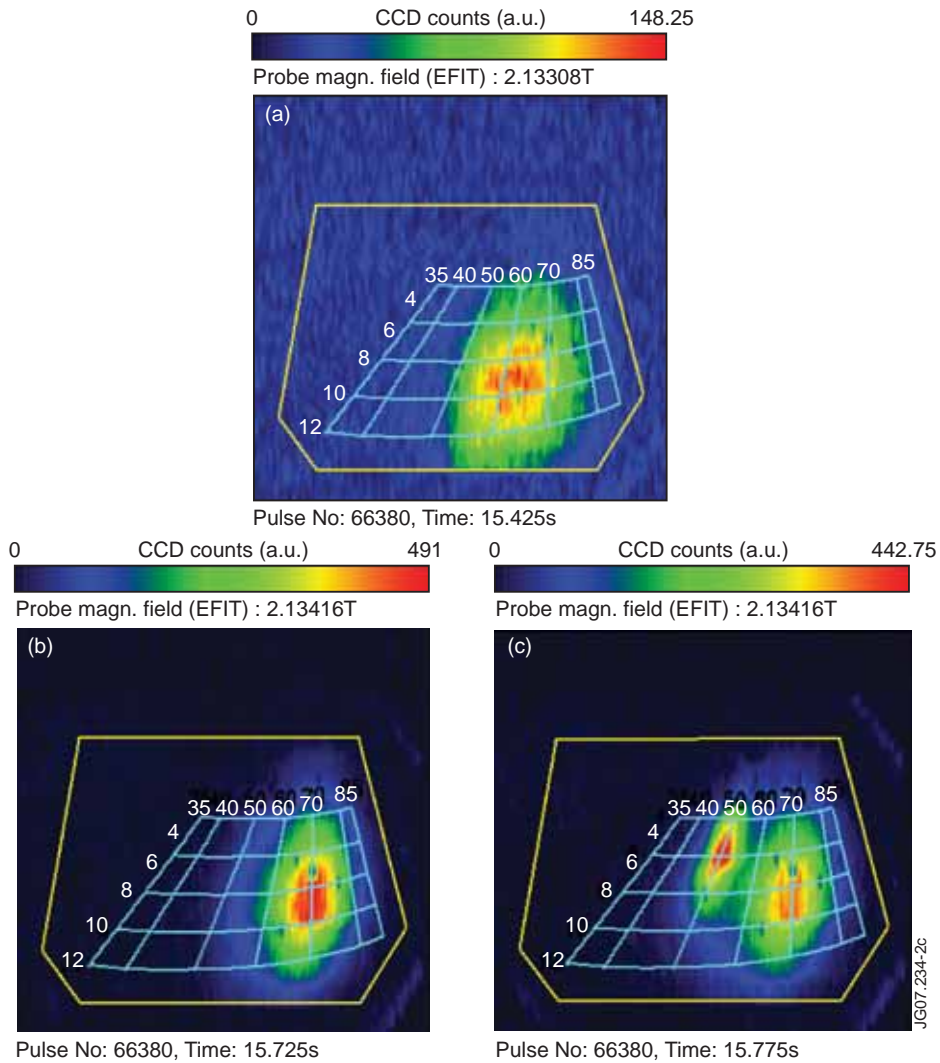
Figure 2 : The three types of measured fast ion losses as function of the pitch angle and gyro radius: before tornado modes are destabilized (left), after tornado modes are destabilized (middle) and during a giant sawtooth crash (right) (Pulse No: 66380).
