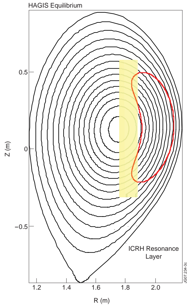
Figure 3: Hags simulation: Typical banana orbit of an ICRH accelerated ion with its banana tips inside the ICRH resonance layer (yellow strip).
