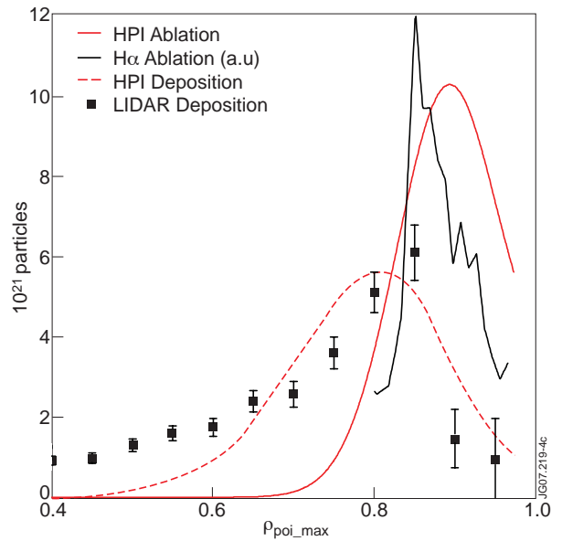
Figure 3: Comparison of the pellet ablation and deposition profiles, calculated with HPI, with the measurement for two representative pellet injections from the LFS (a) and the HFS (b) in the JET experiment Pulse No: 58337.
