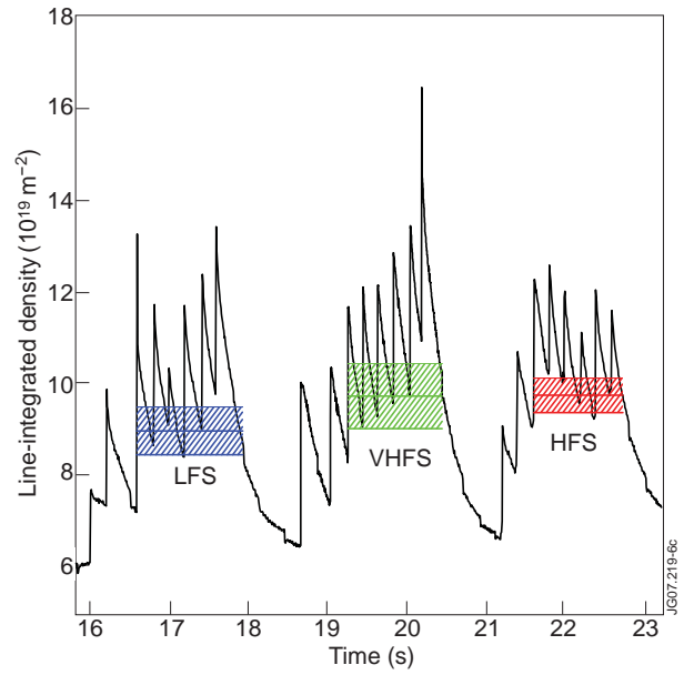
Figure 5: Time evolution of the line-integrated density signal KG1V/LID3 in the JET experiment Pulse No: 58337, and the density equilibrium level for each pellet injection series (blue: LFS, red: HFS), calculated with the averaged local density minima in the equilibrated phase.
