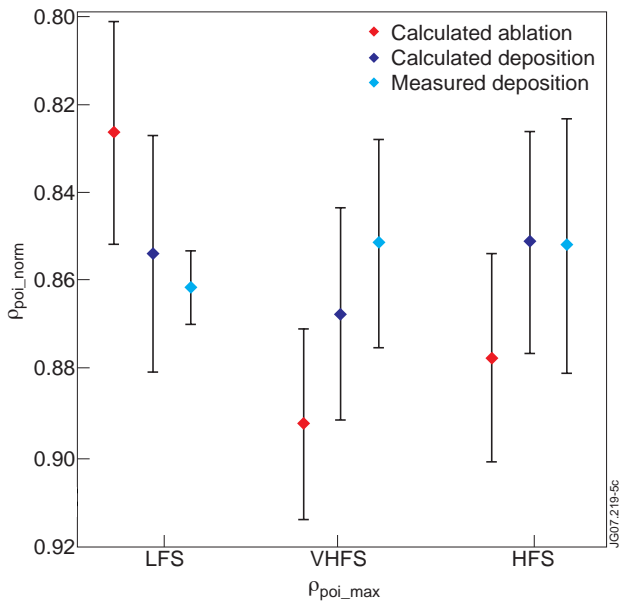
Figure 4: JET experiment Pulse No: 58337, average calculated particle ablation (red) and deposition (blue) barycentres for each pellet injection direction, compared to the average barycentres of the deposition profiles derived from the interferometer signal (cyan).
