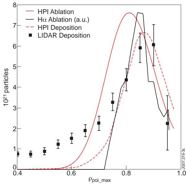
Figure 3: Comparison of the pellet ablation and deposition profiles, calculated with HPI, with the measurement for two representative pellet injections from the LFS (a) and the HFS (b) in the JET experiment Pulse No: 58337.
