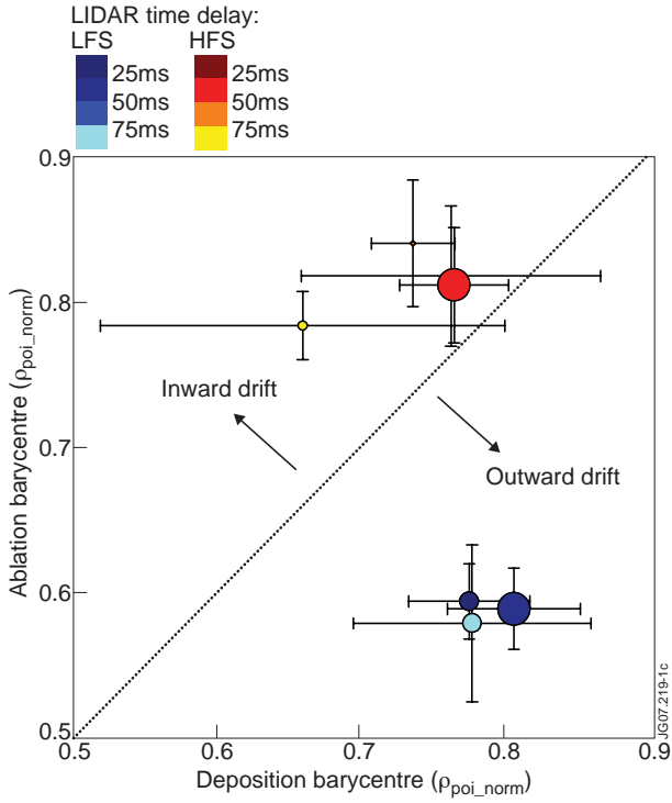
Figure 1: Average barycentres for the pellet ablation and deposition profiles in the JET pellet database, plotted in dependence of the pellet injection direction and the relative timing of the LIDAR. The size of the circles corresponds to the amount of analysed data. The black squares indicate the position of the average barycentres of the JET experiment Pulse No: 58337.
