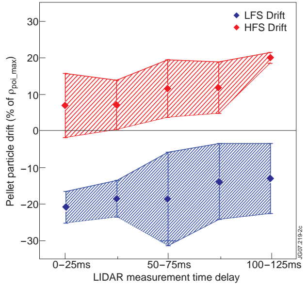
Figure 2: Average pellet particle drift in JET pellet experiments for LFS and HFS injections and its dependence on the LIDAR measurement delay due to particle transport (diffusion etc.).
