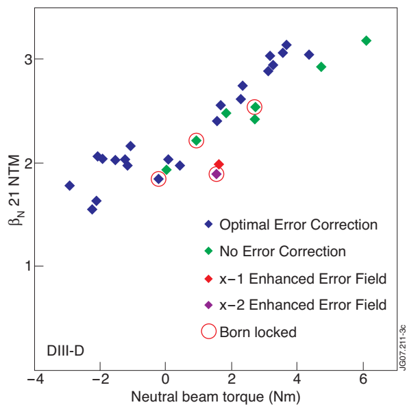
Figure 3: Variation of 2/1 NTM threshold as beam mix is varied from net co- (+ve x) to net counter- injection (-ve x).
