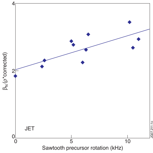
Figure 1: 3/2 NTM threshold variation in ICH:NB scan.
