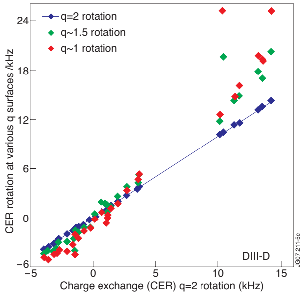
Figure 5: q\sim 1, 1.5, 2 carbon rotation (from charge exchange) at 2/1 NTM onset.
