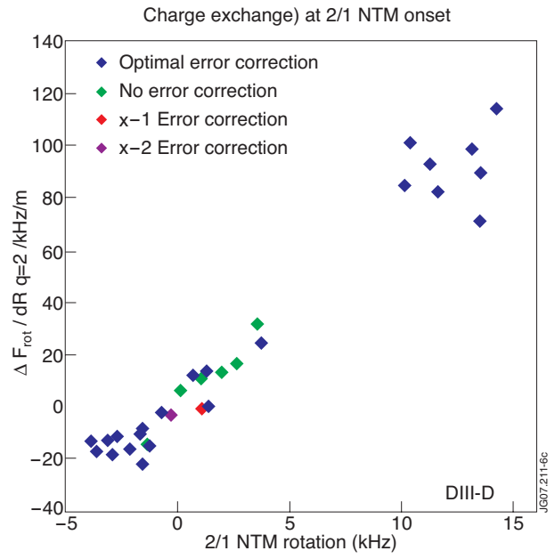
Figure 6: Toroidal rotation gradient at q\sim 2 (carbon) at 2/1 NTM onset.
