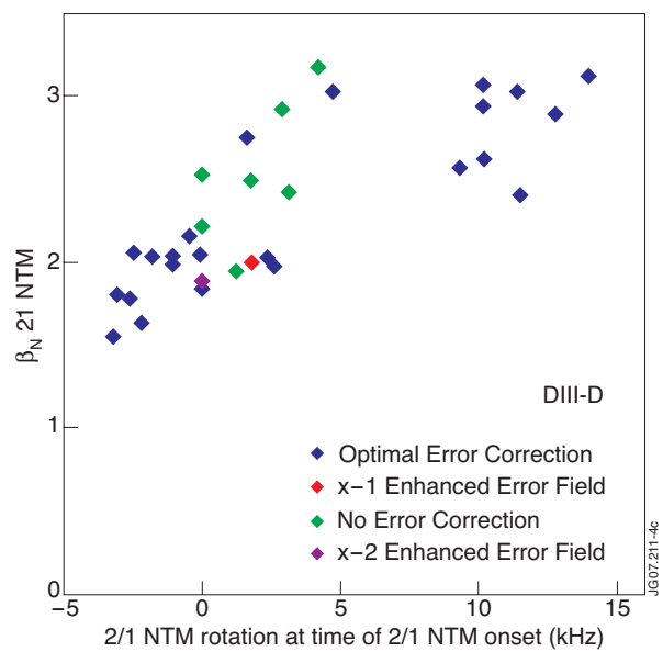
Figure 4: Variation in 2/1 NTM threshold versus mode frequency on DIII-D
