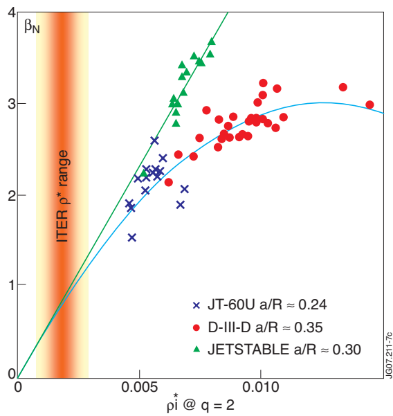
Figure 7: 2/1 NTM hybrid \beta_N limit (and JET stable points) cross machine scaling.
