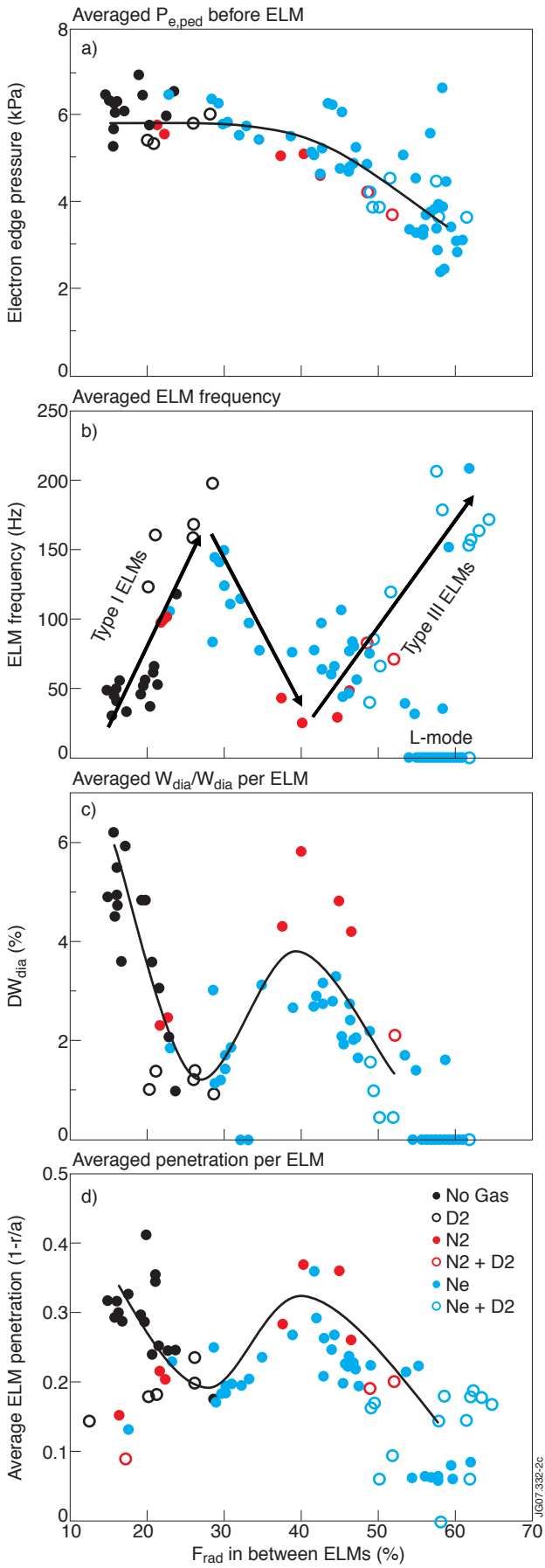
Figure 2: Series 1 (a) Electron Pedestal pressure (b) ELM Frequency (c) averaged diamagnetic energy drop per ELM (d) averaged penetration radius per ELM as a function of radiated power fraction. (ELM penetration is defined as the deepest region in the plasma where \Delta T_{e,ELM}/T_e > 5\% ) Values are time averaged over 1-2s windows.
