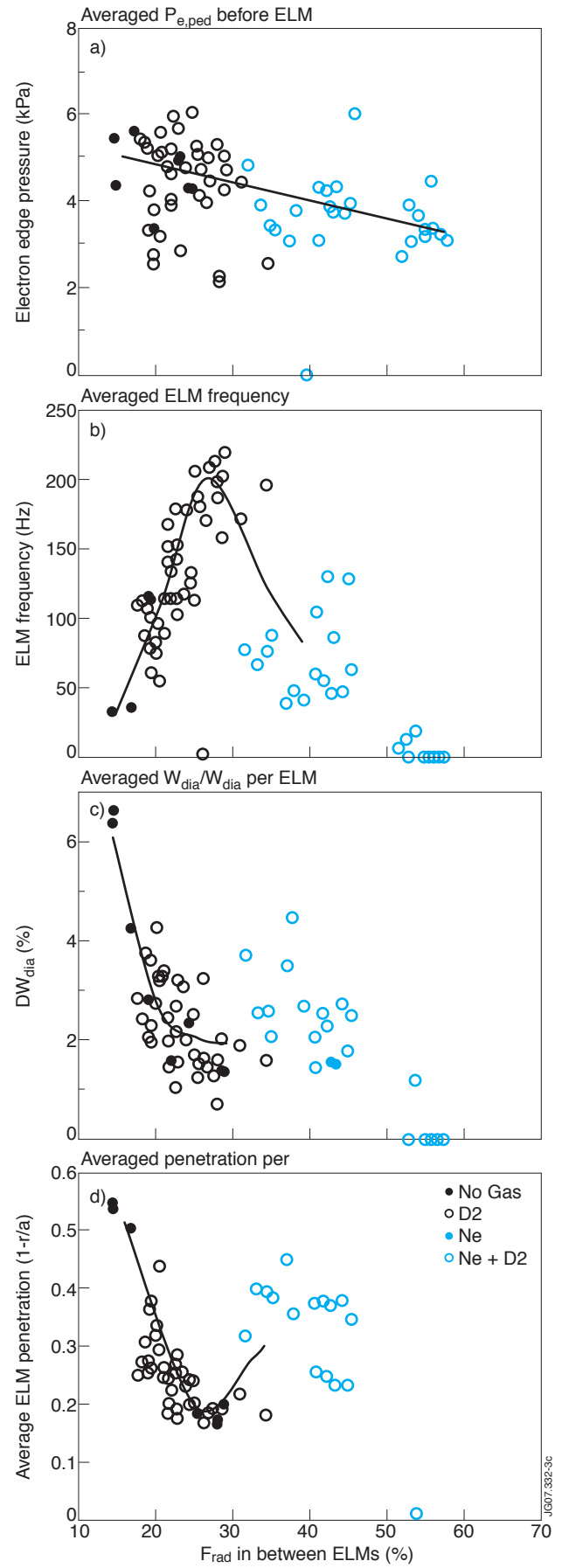
Figure 3: Series 2 (a) Electron Pedestal pressure (b) ELM Frequency (c) averaged diamagnetic energy drop per ELM (d) averaged penetration radius per ELM as a function of radiated power fraction. (ELM penetration is defined as the deepest region in the plasma where \Delta T_{e,ELM}/T_e > 5\% ) Values are time averaged over 1-2s windows.
