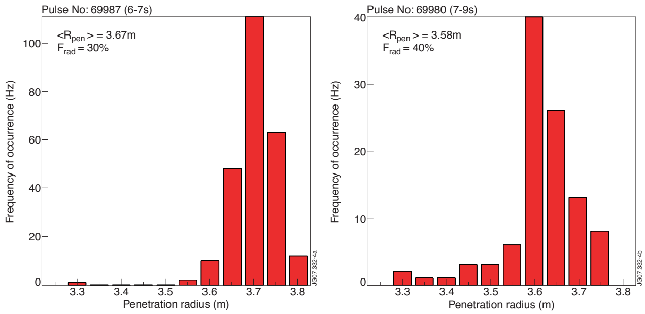
Figure 4: Histogram of Radial ELM penetration for F_{rad} of 30% and 40%
