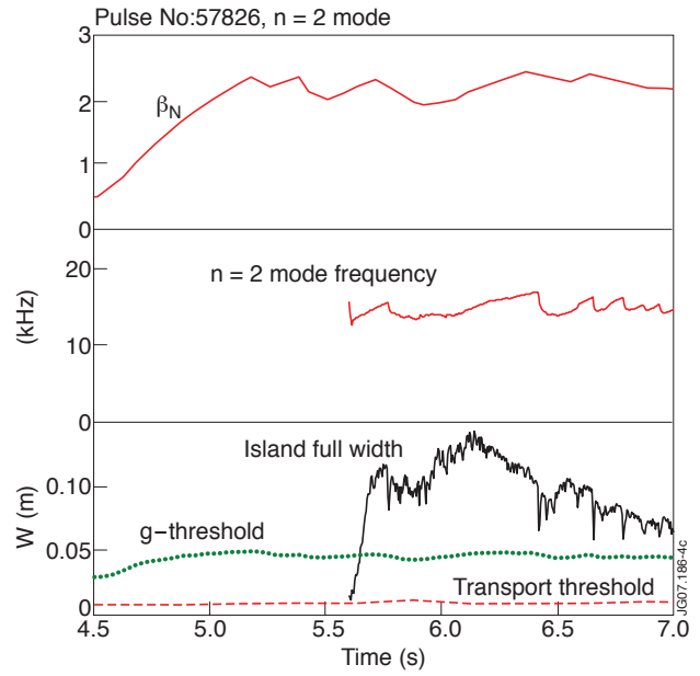
Figure 4: Time history of \beta_N , NTM frequency and island width showing a spontaneous NTM onset. Transport and ion polarisation ( g ) thresholds are shown.
