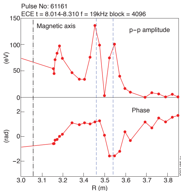
Figure 1: Amplitude and phase of T_e oscillations. Vertical blue lines mark island extremes.
