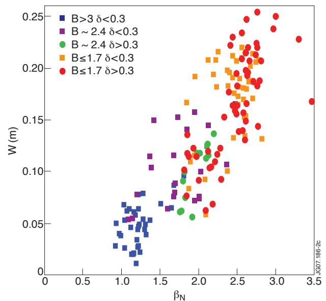
Figure 2: Island width versus normalised beta.
