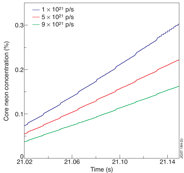
Figure 2: Neon concentration in the plasma core for three deuterium puffs levels, 1 \times 10^{21} p/s; 5 \times 10^{21} p/s and 9 \times 10^{21} p/s and H-mode plasmas.
