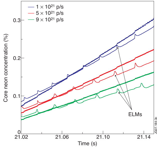
Figure 3: Neon concentration in the plasma core for three deuterium puffs levels, 1 \times 10^{21} p/s; 5 \times 10^{21} p/s and 9 \times 10^{21} p/s and H-mode plasmas with (continuous line) and without ELMs (shaded line)
