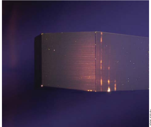
Figure 5: Photograph of two tiles (height 80mm) during heat loading in GLADIS. The bright horizontal features are fibre planes perpendicular to the surface. The bright vertical features on the right-hand tile are developing tensile cracks. The power density is centered in the middle of the tiles.
