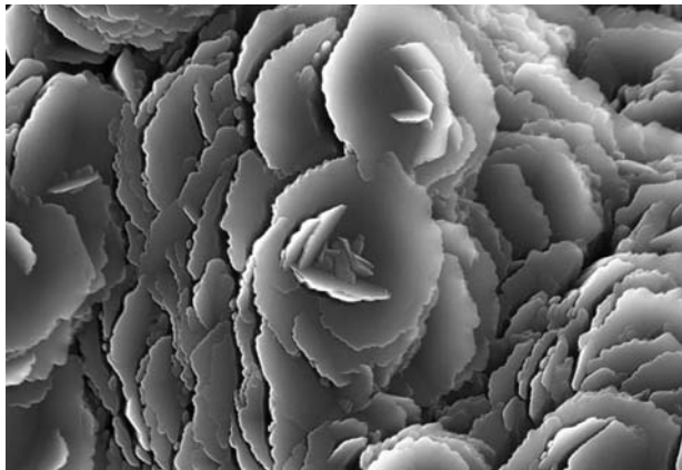
Figure 1: Details of surface structure of the evaporated Be layer deposited on cast Inconel.
