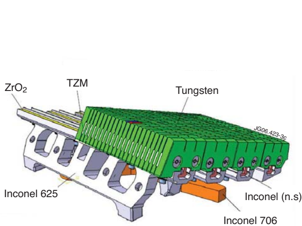
Figure 3: Left: Bulk W lamellae concept (only one half shown with W lamellae in place): Right: Cross-section of the JET divertor showing the locations of bulk (blue) and coated solutions (red).
