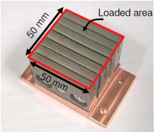
Figure 4: Bulk tungsten test tile for high heat flux tests in the Judith facility.
