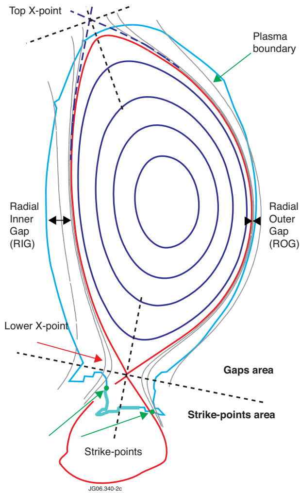
Figure 2: Plasma geometry identification. X-points top and lower, gaps, strike points are some of the objects identified by Felix.
