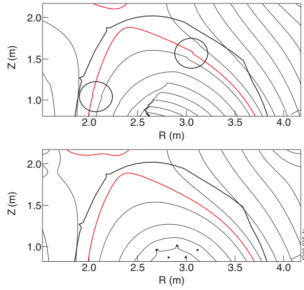
Figure 4: Comparison between Taylor expansion model (left) and filamentary model (right) boundary reconstructions.
