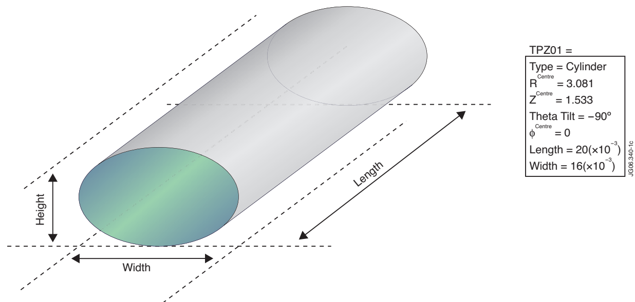
Figure 1: Coil model approximation and equivalent description using the rules adopted in the MCF Geometry group.
