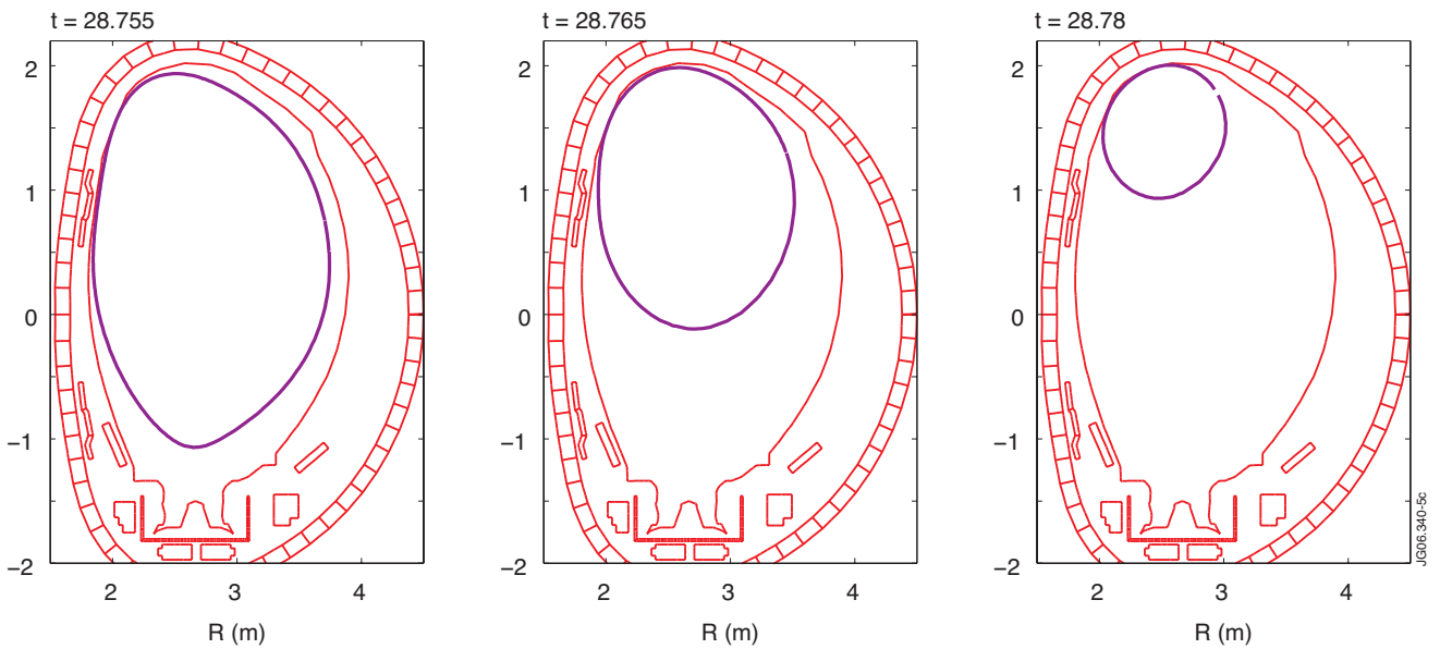
Figure 5: Reconstruction of the evolution of the plasma shape during a disruption obtained using the CREATE model.
