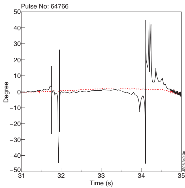
Figure 3: X-Point rotation angle. Old model XLOC (-) and new expansion model (-, -).
