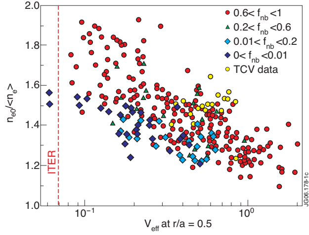
Figure 1: Density peaking versus effective collisionality in JET H-modes, resolved by the fraction of NBI heating, f_{\text{nb}} = P_{\text{NB}}/P_{\text{tot}} . Purely electron heated TCV points are also included.
