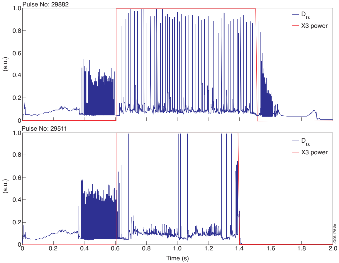
Figure 2: X3 heated H-mode scenarios: (a) with giant ELMs (b) with stationary ELM-free phases
