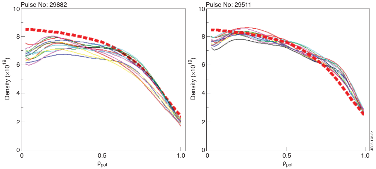
Figure 3: Multiple TS measurements of density profiles during X3 heating for ELMy (a) shot and ELM-free (b) shot. Red dashed line – density profile in an Ohmic H-mode plasma.
