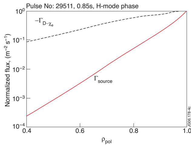
Figure 4: Kn1D simulation of edge neutrals flux and comparison with particle diffusion flux for X3 heated H-mode plasma on TCV.
