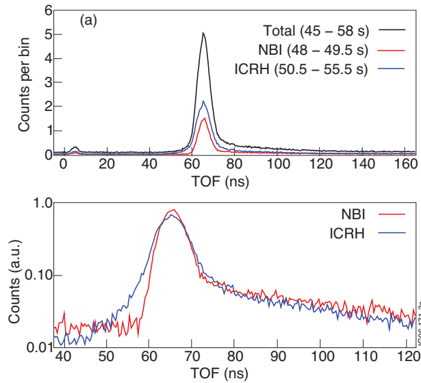
Figure 3: Neutron time-of-flight spectra. (a): Raw TOF spectra. One time bin corresponds to 0.4ns. (b): TOF spectra from the the early (NBI dominated) and late (ICRH dominated) period of the discharge. Curves are normalised to to the same intensity.
