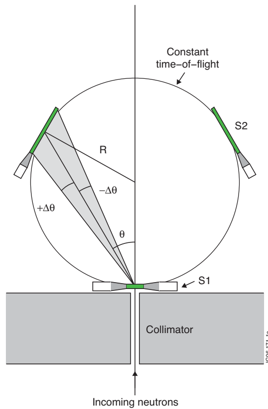
Figure 1: TOFOR principle. The energy of the incoming neutrons is given as a function of the flight time between the S1 and the S2 detectors.
