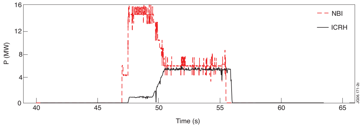
Figure 2: NBI and ICRH heating power for JET Pulse No: 66463.
