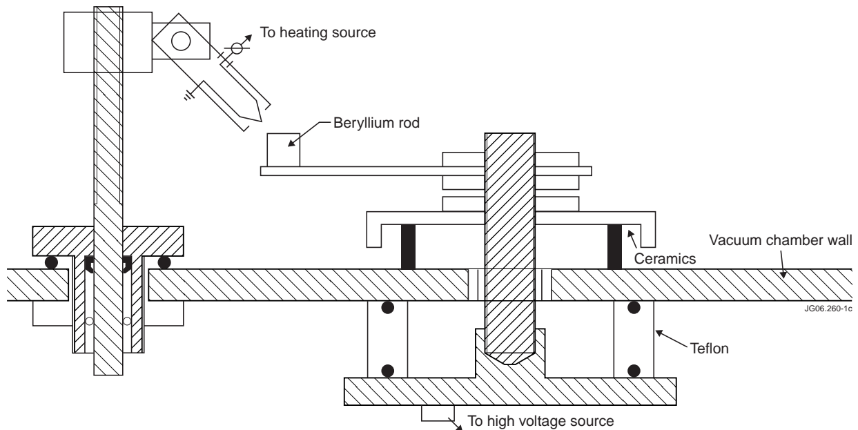
Figure 1: Experimental set-up of the thermionic vacuum arc method for beryllium film formation.
