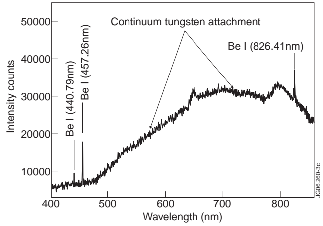
Figure 3: Optical emission spectrum of Be plasma
