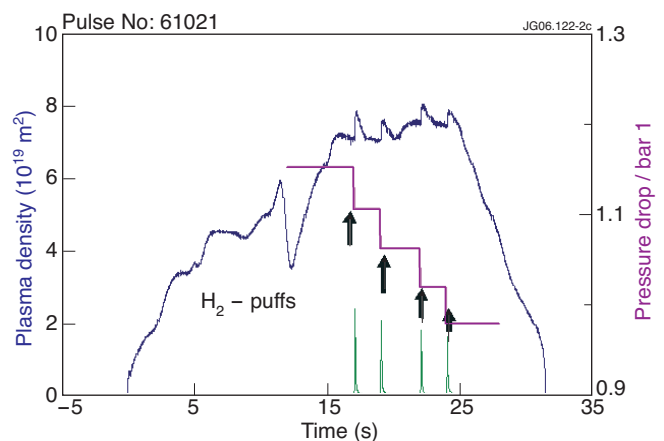
Figure 2a: Hydrogen puffs into a D-plasma at 17, 19 and 22, 24 into the L-mode and Hmode phases of the JET Pulse No: 61021.
