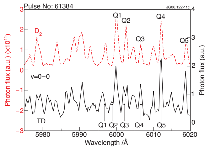
Figure 3e: D_2 spectra before and TD spectra from the 2. line of sight of KT3B during the T_2 puff shown in a).
