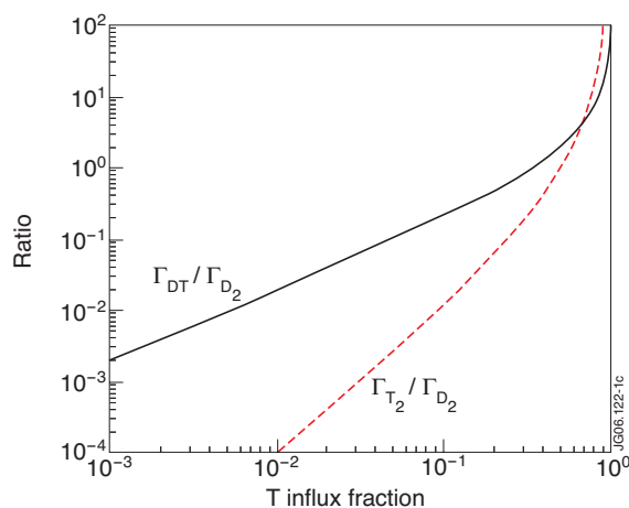
Figure 1: Molecular flux ratios versus surface concentration derived from the law of mass action.
