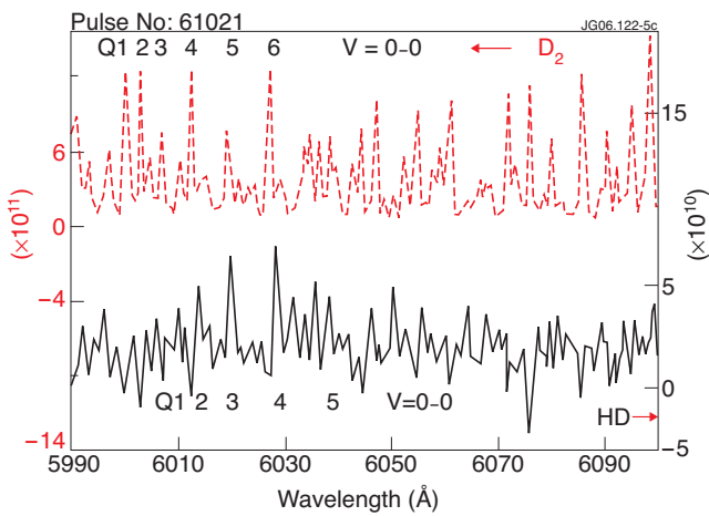
Figure 2d: D_2 spectra before and HD spectra from the 2. line of sight of KT3B during H_2 puffs. The HD spectra are averaged over all puffs in a).
