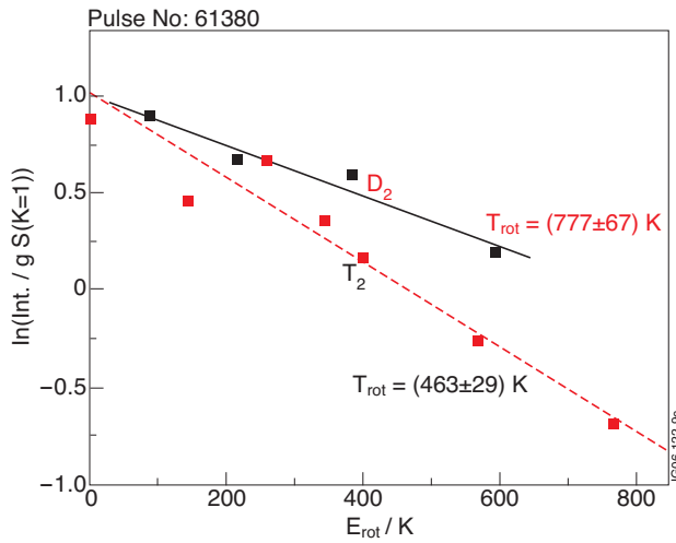
Figure 3c: Plot of the rotational intensity distributions versus their level energies for D_2 and T_2 shown in a).
