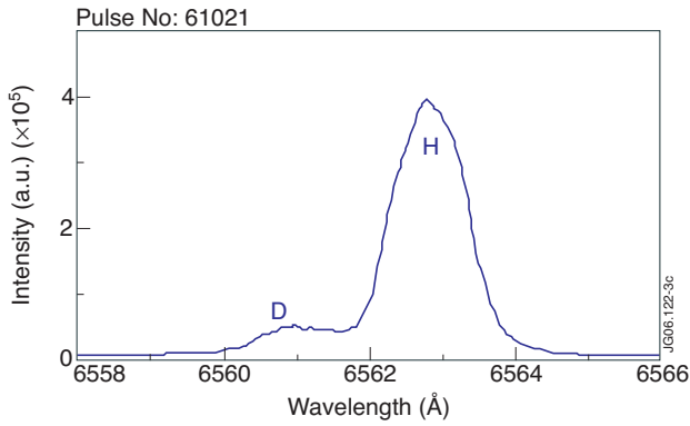
Figure 2b: H and D Balmer- \pm lines near their injection port GIM 15 at octant 6.
