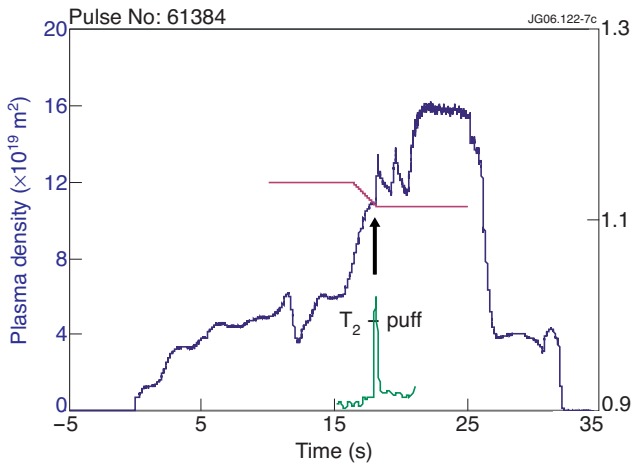
Figure 3a: A tritium puff into a D-plasma during the L-mode phase of JET Pulse No: 61384.
