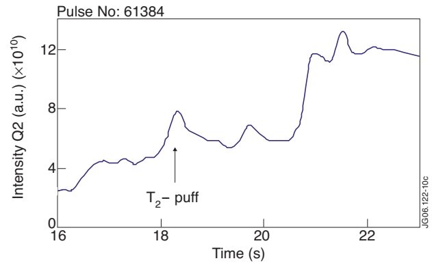
Figure 3d: TD release from the intensity of the Q2-line versus time in the outer divertor during the injection shown in a).
