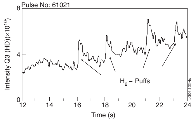
Figure 2c: HD release from the intensity of the Q3-line versus time in the outer divertor during the injections shown in a)
