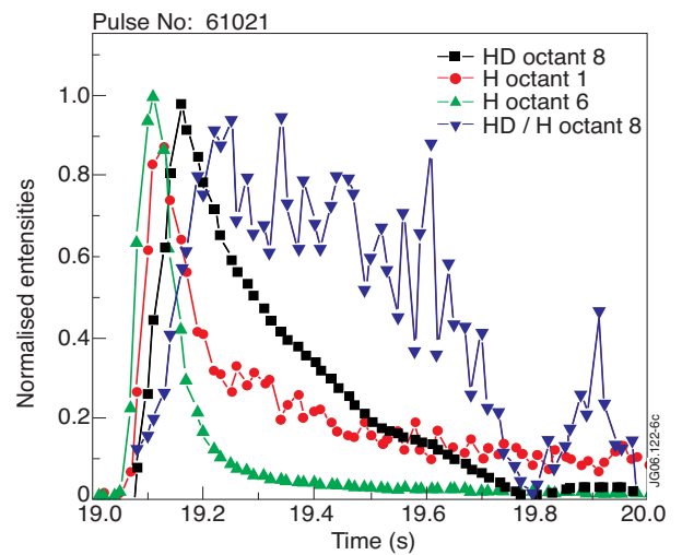
Figure 2e: The H\nu puff at 19s and the respective responses of the hydrogen atoms and HD molecules in the outer divertor during the L-mode as well as the resulting HD/H intensity ratio.
