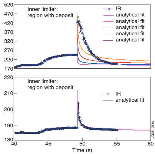
Figure 4: Temperature evolution of 2 positions on the limiter tile: with and without a deposited layer.
