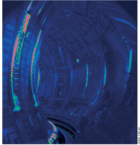
Figure 2: Visible (left) and infrared images during the disruption of a plasma contacting the inner limiters.
