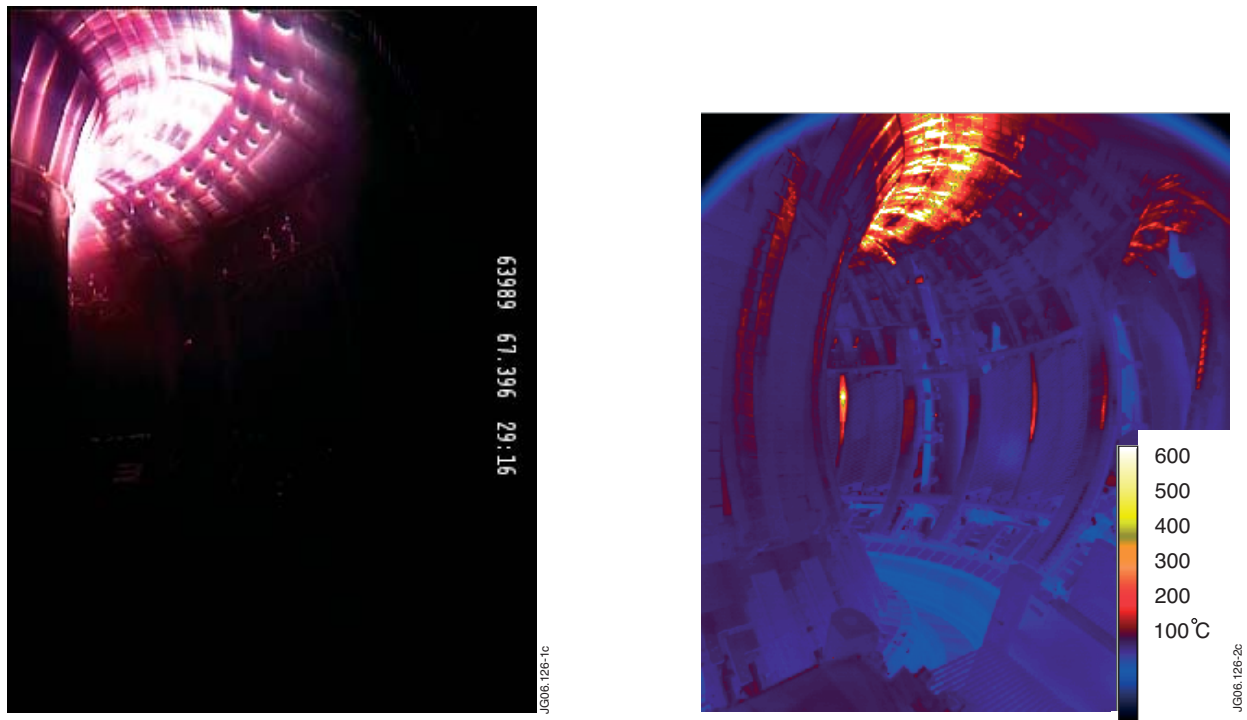
Figure 1: Visible (left) and Infrared images during the disruption of a vertically displaced plasma.
