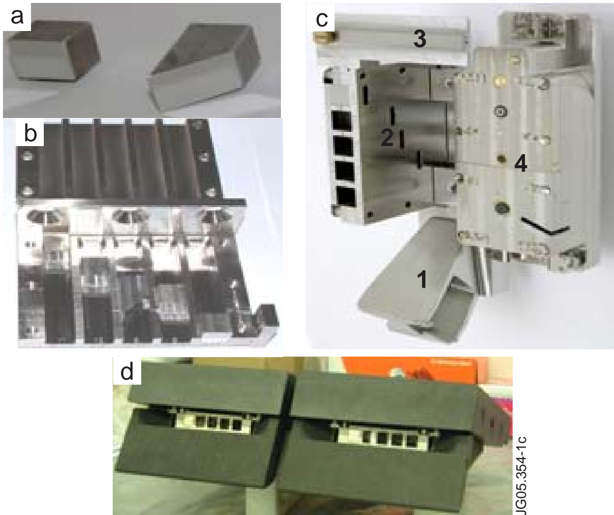
Figure 1: Components for the FMT and TRS at JET: (a) flat front and angled molybdenum mirrors; (b) open cassette with mirrors; (c) bracket assembly for installation on the main chamber wall: 1. wall bracket; 2. cassette with mirrors; 3. magnetic shutter; 4. rotatable deposition monitor; (d) cassettes installed in the divertor base.
