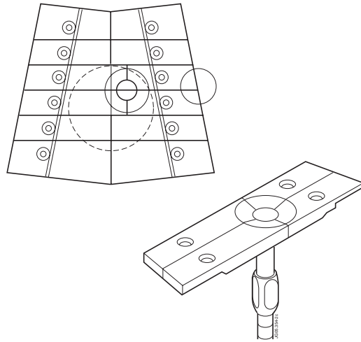
Figure 2: Schematic drawings showing the installation of the sample manipulator in the TCV vessel floor.
