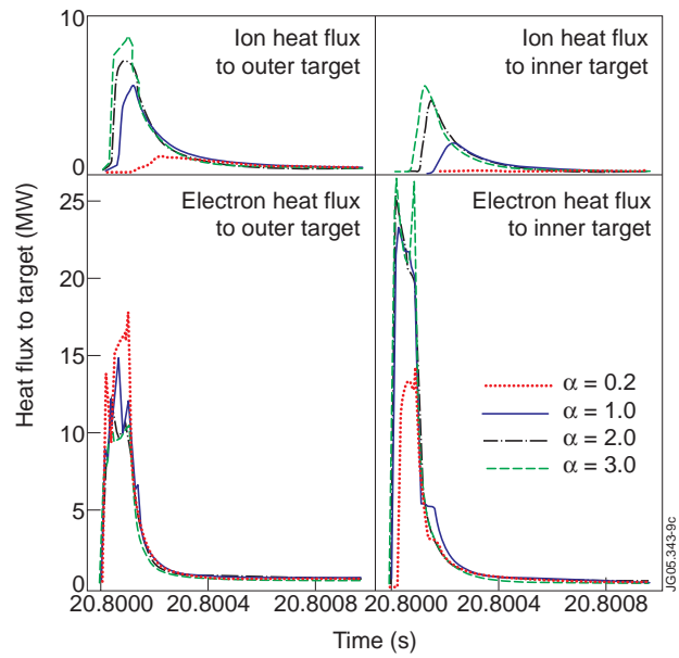
Figure 4: Ion and electron heat fluxes at the outer and inner targets for four different values of the parallel heat flux limiting factors.
