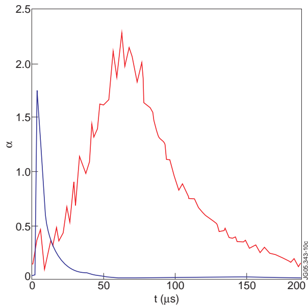
Figure 5: The parallel flux limiting factors \alpha_i (red curve) and \alpha_e (blue curve) as a function of time during an ELM in a low-recycling JET plasma.
