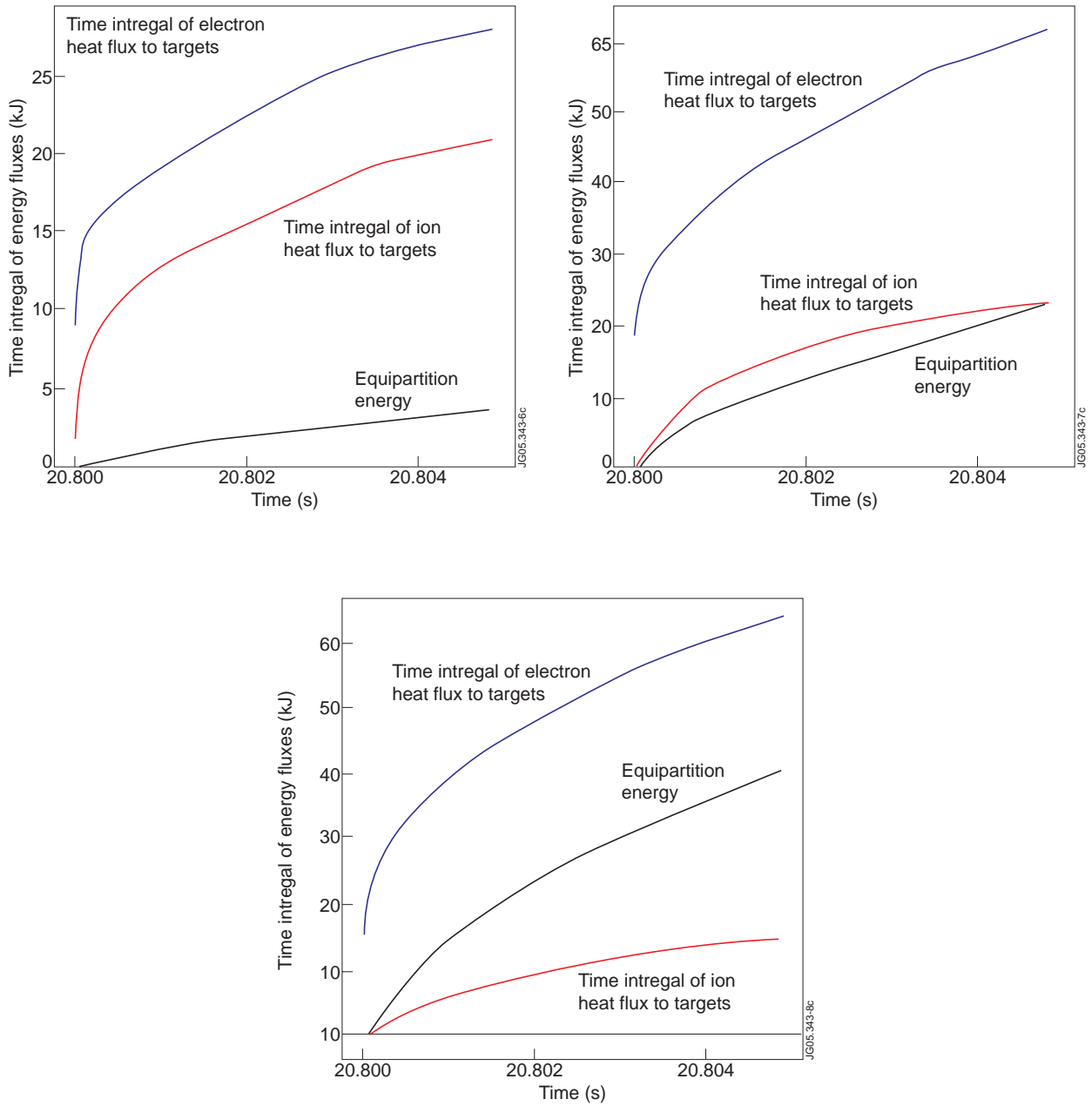
Figure 3: Time integrals of the total ion heat flux measured at both targets, the total electron heat flux measured at both targets and the volume-integrated ion-electron equipartition energy as a function of time for three simulations with the following separatrix densities: (a) 8 \times 10^{18} \text{ m}^{-3} , (b) 1.7 \times 10^{19} \text{ m}^{-3} and (c) 4.0 \times 10^{19} \text{ m}^{-3} .
