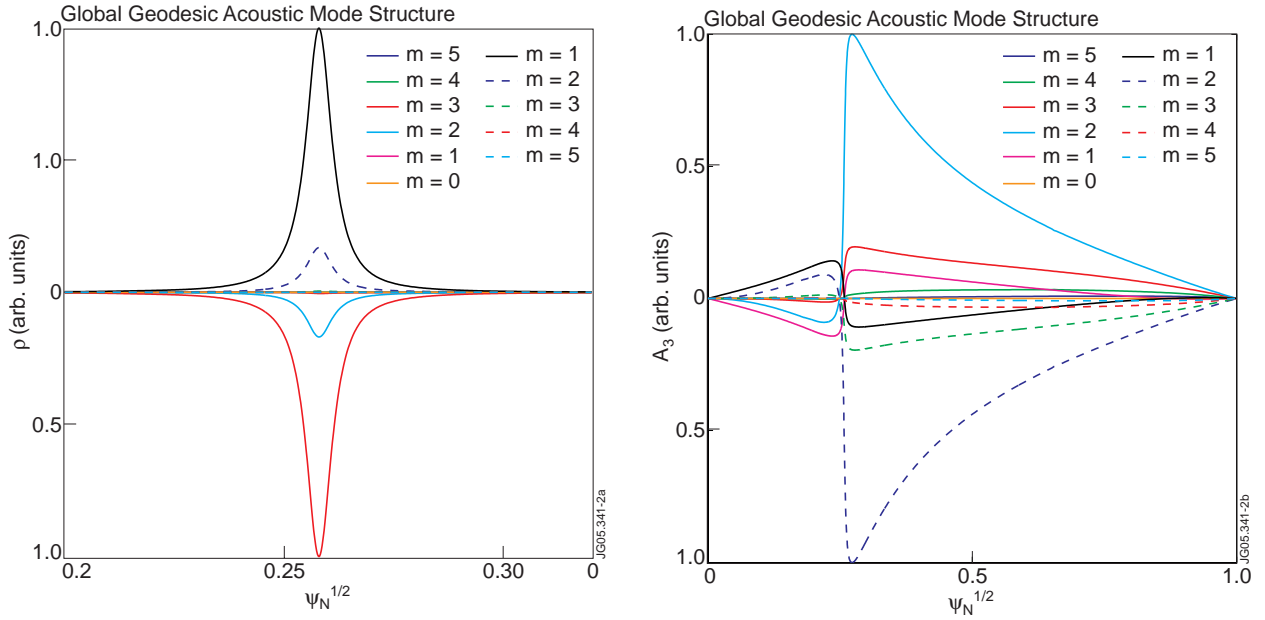
Figure 2: Eigenmode structure of the global geodesic acoustic mode found slightly above the peak in the geodesic acoustic wave continuum, located at \sqrt{\psi_N} = 0.26 , for a reversed shear, circular JET-like equilibrium. (a) The perturbed mass density and (b) the perturbed parallel vector potential.
