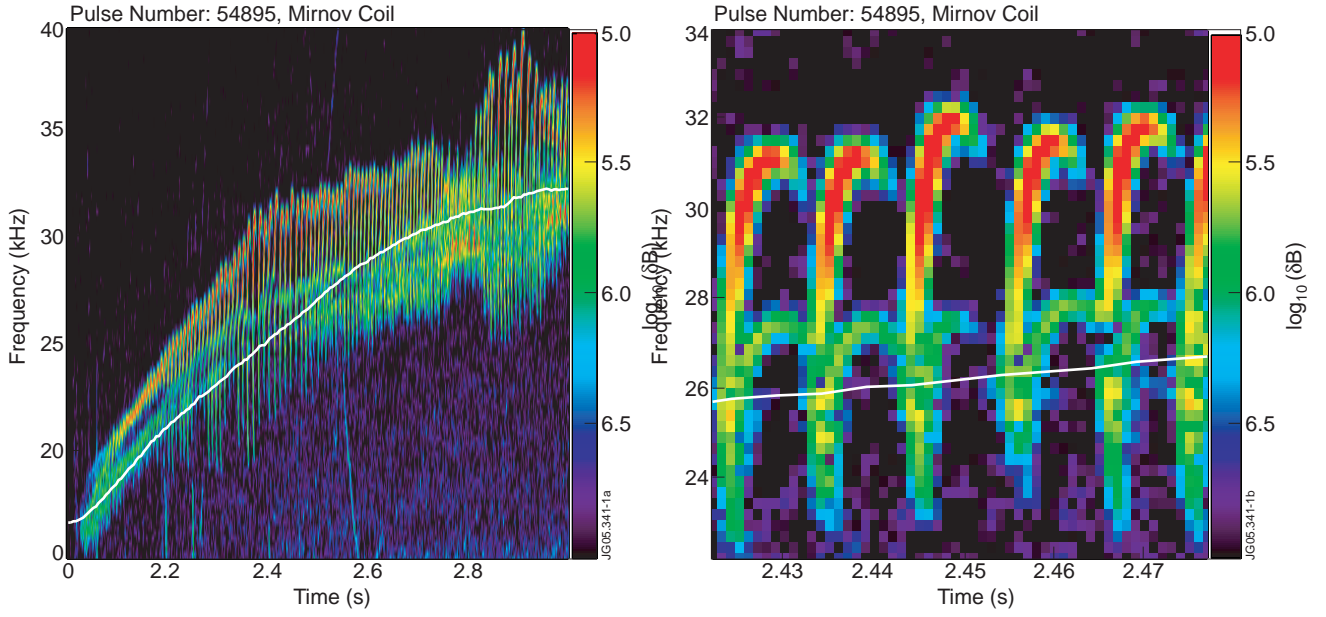
Figure 1: Spectrograms of the signal from a Mirnov coil on JET. (a) The rapidly chirping n = 0 mode. (b) A zoom of (a) showing the frequency chirping in more detail. In both plots the white line is proportional to \sqrt{T_e}(r/a = 0.15) .
