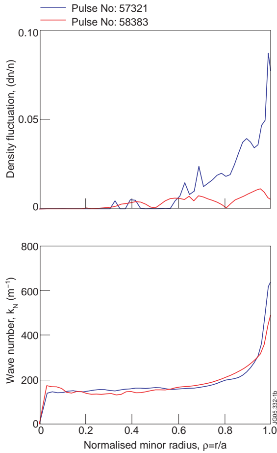
Figure 1: Comparison of the main plasma and heating parameters versus time for the Pulse No's:57321 and 58383 from the experiments (left). On the right-hand side a comparison of the density fluctuations and the perpendicular wave number calculated by the model presented in this paper is shown for the same shots at t=3.7s for Pulse No:58383 and t=13.4 for Pulse No: 57321.
