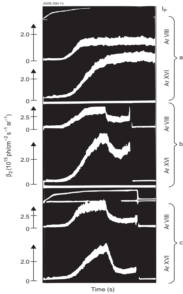
Figure 1: Time evolution of radiance B_z of Ar^{7+} and Ar^{15+} : a) Ohmic discharge b) RF pulse on n_H/n_D = 0.685 c) RF pulse on n_H/n_D = 0.485 . Data from Ref. [1]
