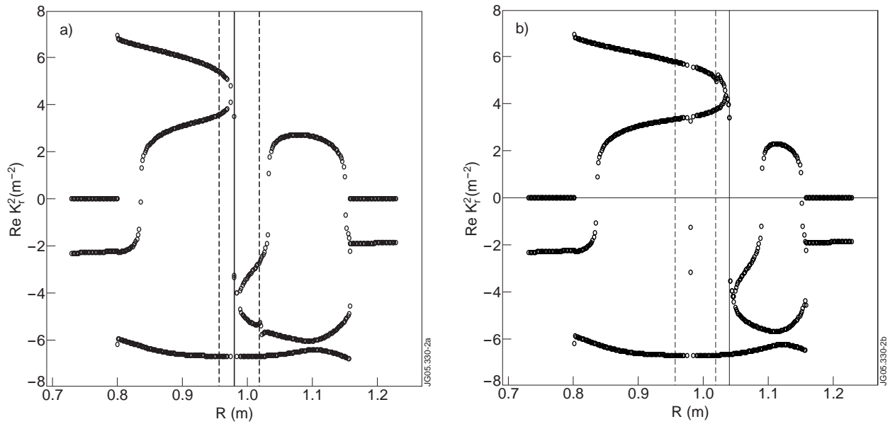
Figure 2: The radial profiles of k_{\perp}^2 for different concentration ratio a) n_H/n_D = 0.69 , b) n_H/n_D = 0.47 .
