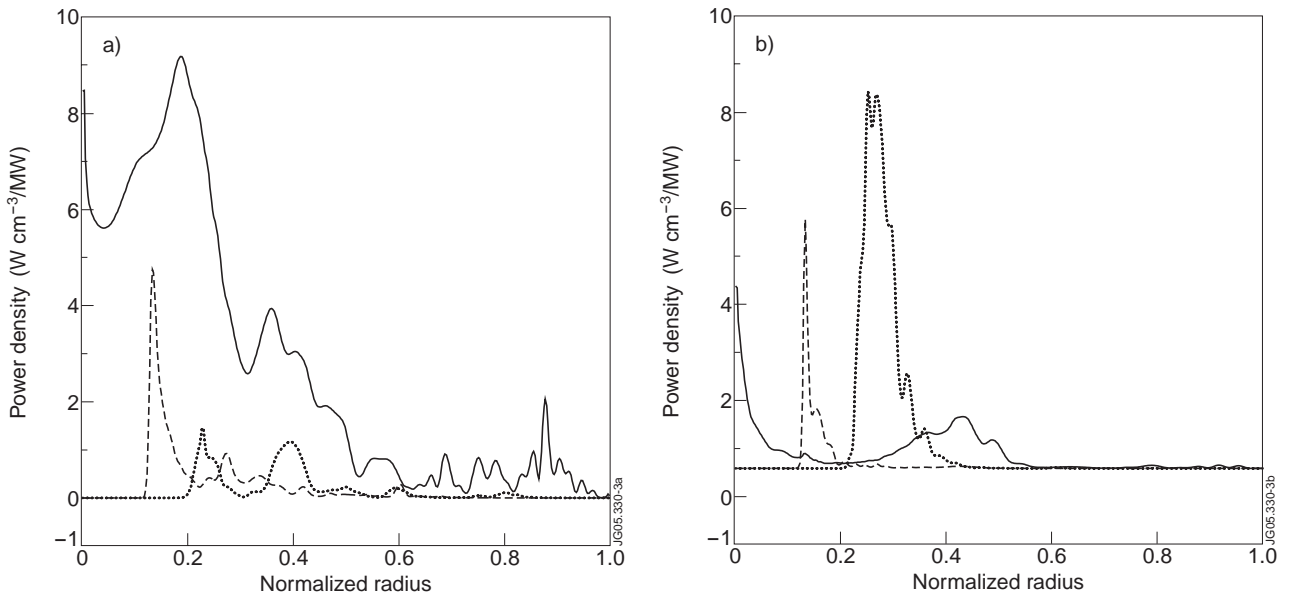
Figure 3: The radial profiles of absorbed power by electrons (solid line), Ar 15+ (dash line), Ar 16+ (dot line). Case a) n_H/n_D = 0.69 , b) n_H/n_D = 0.47 .
