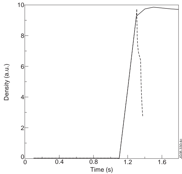
Figure 4: The time evolution of the total argon concentration in case density ratio n_H/n_D = 0.47 : without ripple losses (solid line), with ripple losses (dash line).
