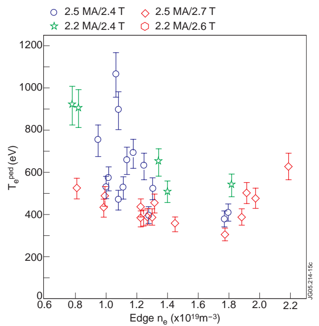
Figure 2: P_{th} and corresponding pedestal T_e^{ped} values plotted as a function of the edge n_e for MkiIGB Septum divertor.
