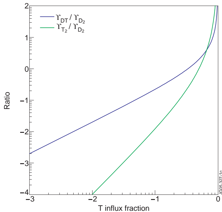
Figure 1: Molecular flux ratios versus surface concentration
