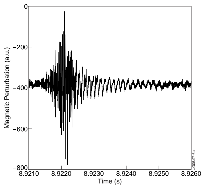
Figure 6: Temporal evolution of B_{\sim} for a single burst of hybrid fishbones (Pulse No: 54300).
