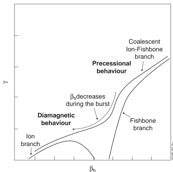
Figure 5: Schematic diagram of the solutions of the dispersion relation (5): Mode growth rate as function of the fast particles beta.
