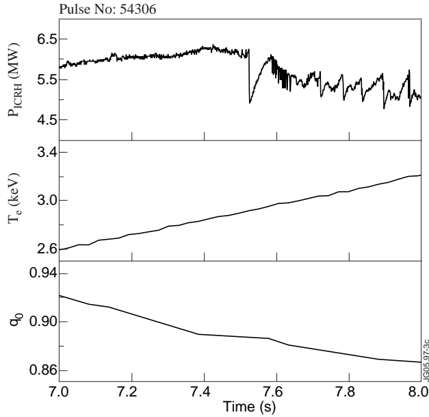
Figure 3: Temporal evolution of the electronic temperature, ICRH power and safety factor on axis during the RF ramp phase in Pulse No: 54306
