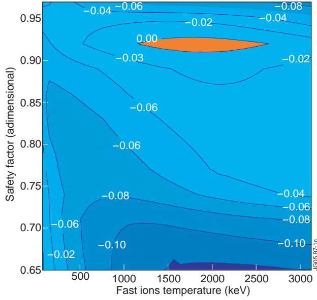
Figure 1: Perturbation on the kink mode growth rate due to the non adiabatic part \delta W_{HOT}^{na} as function of the fast ions temperature and safety factor on axis for a fast ions profile peaked in the center. Blue regions are stabilizing and red destabilizing.
