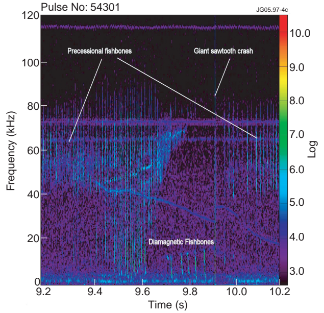
Figure 4: Spectrogram of MHD activity in Pulse No: 54301
