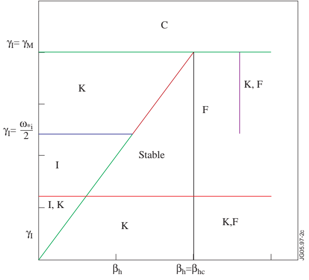
Figure 2: Regions of stability for the different branches of the internal kink dispersion relation in the space of parameters (\gamma_1, \omega_{*i}, \beta_h) . In regions labelled with a K the kink branch is unstable, with an I the ion branch is unstable and with an F the fishbone branch is unstable. In region C the fishbone branch coalesces with one of the low frequency branches (in this case the kink branch).
