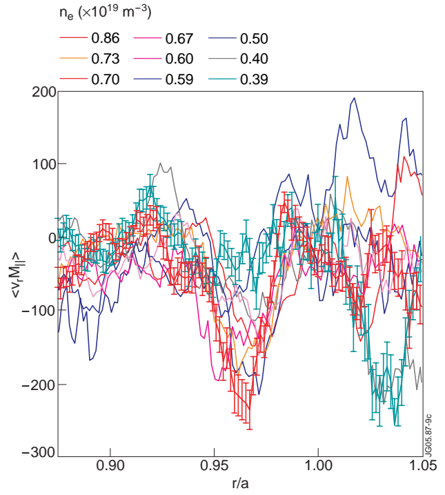
Figure 7: Radial profiles of the cross-correlation between parallel and radial fluctuating velocities in TJ-II plasmas near the LCFS at different plasma densities.
