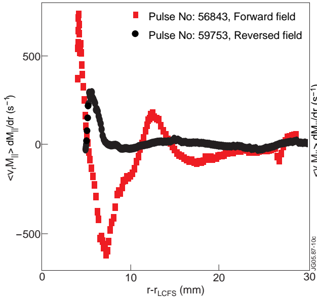
Figure 8: Radial profile of production term in JET.
