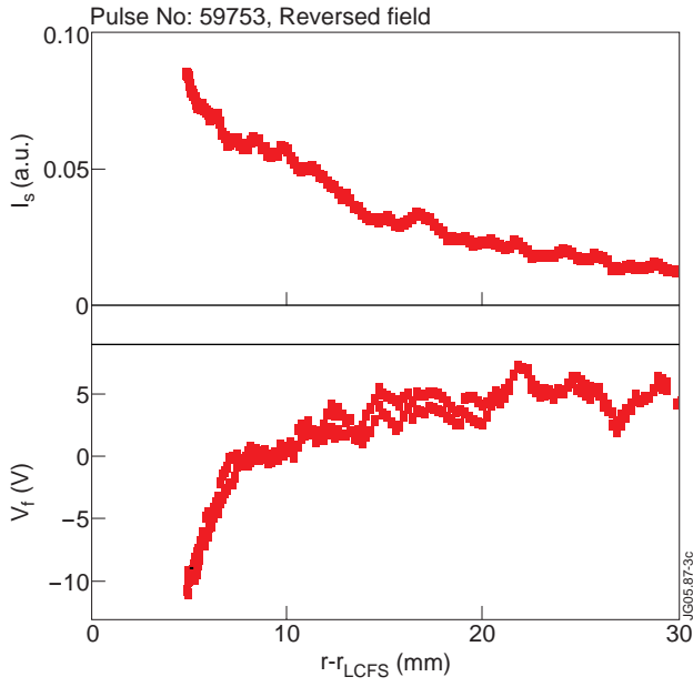
Figure 3: Ion saturation current and floating potential profiles in a reversed field discharge near the LCFS. The probe position is mapped to the outside mid-plane. Measurements were taken in reversed magnetic field configuration at the JET top region.
