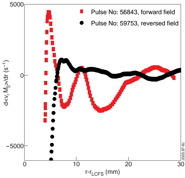
Figure 6: Gradients in the cross-correlation between parallel and radial fluctuating velocities in JET in forward and reversed toroidal field discharges.
