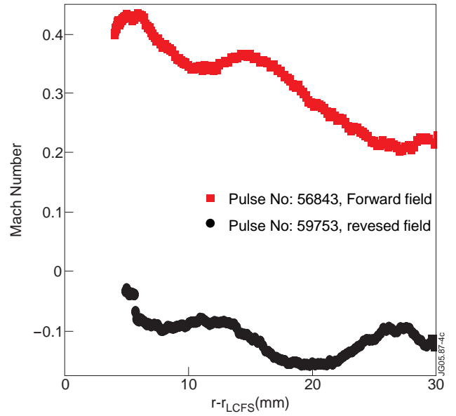
Figure 4: Comparison of Mach number profiles between a forward and reversed toroidal field discharges in JET.
