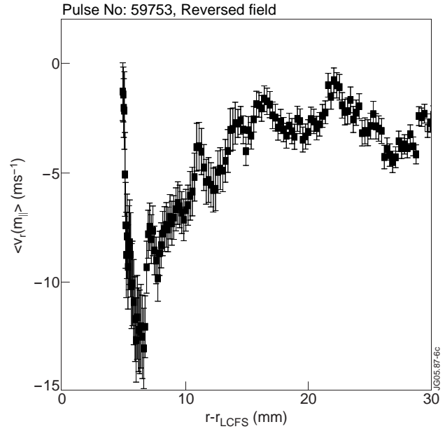
Figure 5. Radial profiles of the cross-correlation between parallel and radial fluctuating velocities in JET L-mode plasmas near the LCFS in forward and reverse field discharges.
