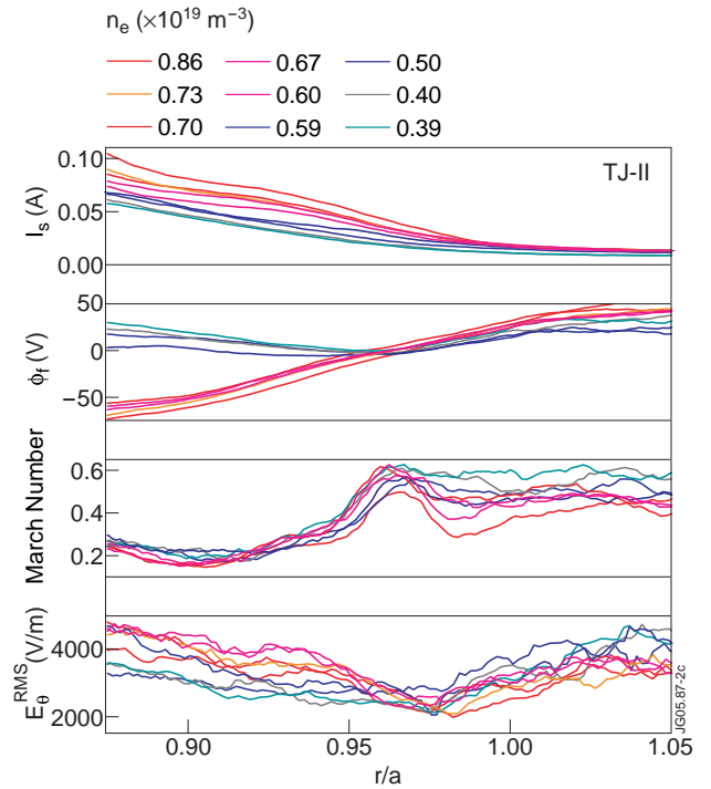
Figure 2: Profiles of ion saturation current, floating potential, parallel flows and level of fluctuations. The experiments were performed in the same configuration and the plasma density was increased in a shot-by-shot basis. The plasma density was increased from 0.3-0.8 \times 10^{19} \text{ m}^{-3} .
