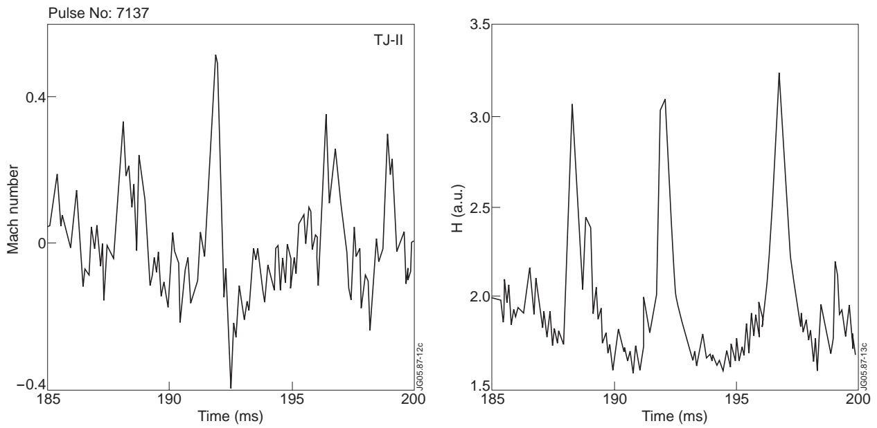
Figure 10: Time evolution of parallel flows and edge instabilities in TJ-II
