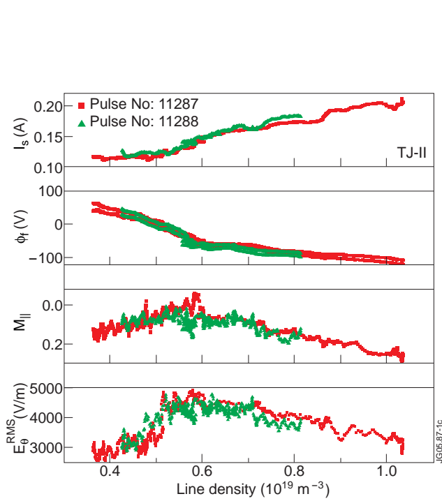
Figure 1: Ion saturation current, floating potential, parallel flows and level of edge fluctuations versus plasma density in the plasma boundary of the TJ-II stellarator. Measurements were taken near \rho \approx 0.85 .
