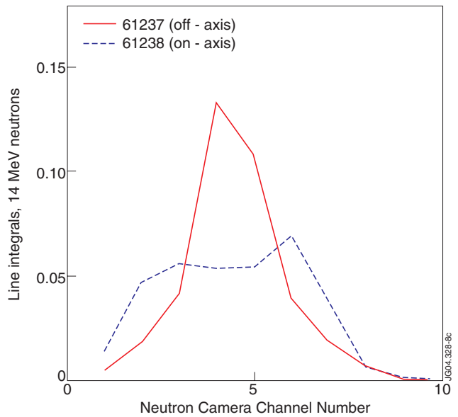
Figure 8: Differences in shape and emissivity centres between on- and off- axis Tritium beam blips.
