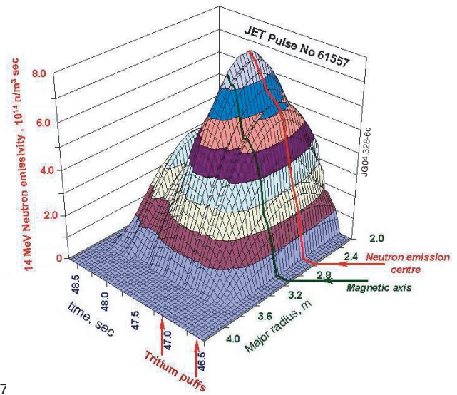
Figure 6: 14MeV neutron profile with ICRH Tritium fundamental heating showing that the neutron emission centre is shifted toward the high field side with respect to the magnetic axis.
