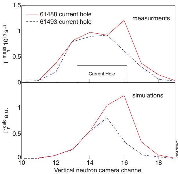
Figure 7: Comparison of calculated and measured profiles for the vertical 14 MeV neutron camera for on-axis tritium beams. DT neutron profiles during on-axis tritium beam blip indicate an outward displacement of neutron emission (measured on the top, calculated on the bottom).
