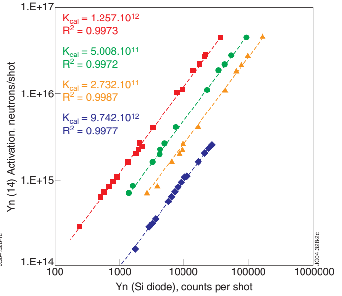
Figure 2: Calibration factors for four different Silicon diodes (DT neutron monitors) derived from activation measurements.
