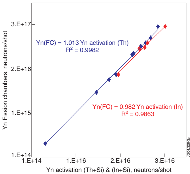
Figure 3: Cross calibration of fission chambers against activation system for DD plasma: in red
