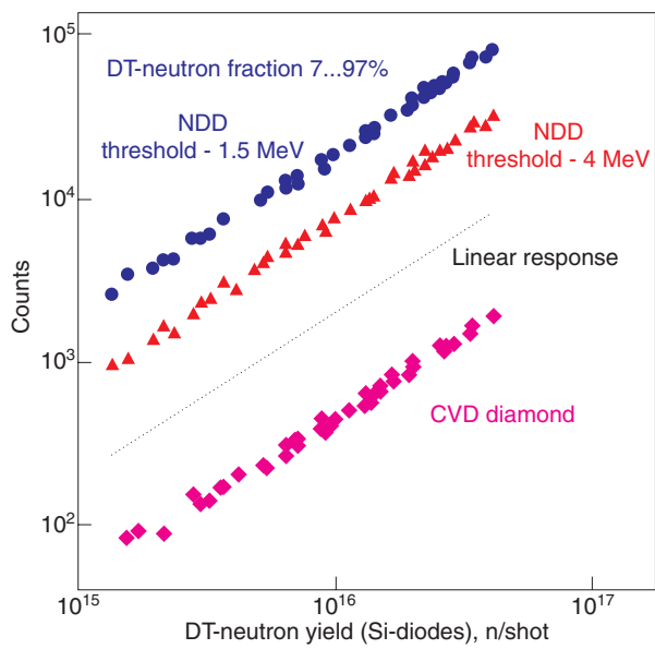
Figure 1: NDD and CVD Diamond detectors response to Tritium JET Pulse No's: 61084-61236
