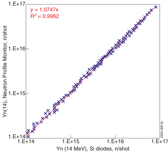
Figure 5 Comparison of 14MeV neutron yield measured by Neutron Profile Monitor (Bicron detectors) and Si diodes (~450 TTE shots)
