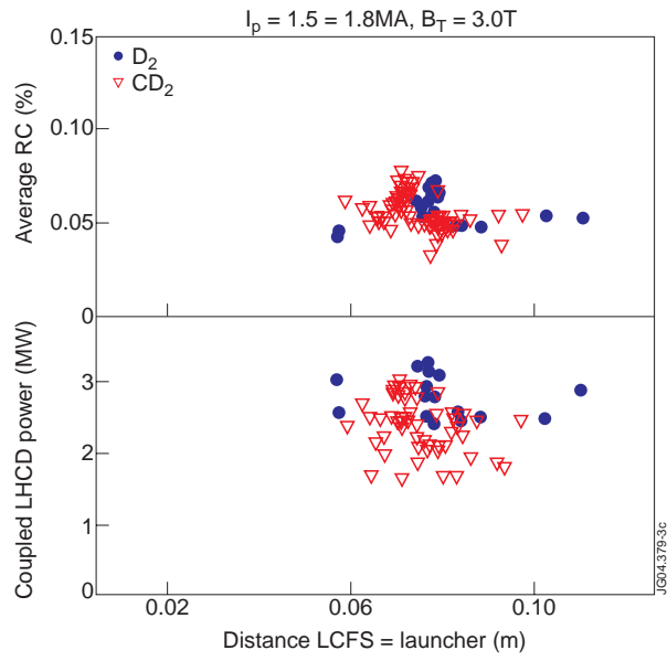
Figure 3: Overview of LH coupling behaviour with CD_4 and D_2 .
