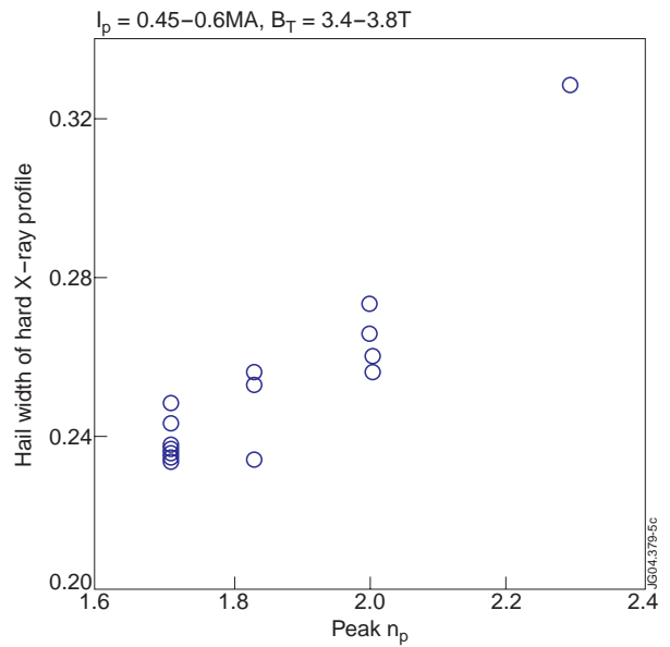
Figure 5: Half width of hard X-ray profile versus peak n_{||} value.
