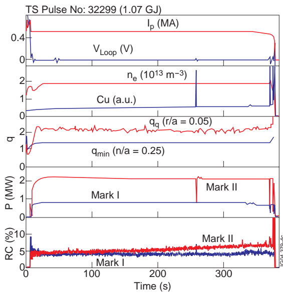
Figure 4: Tore Supra discharge with IGJ injected energy.
