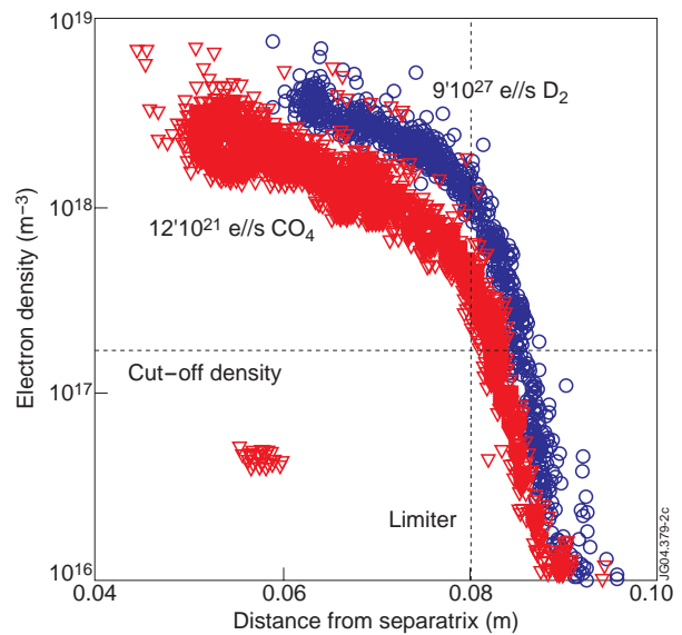
Figure 2: Effect of CD_4 and D_2 on the scrape-off layer electron density.
