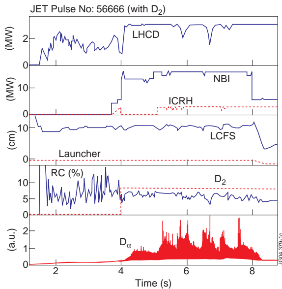
Figure 1: LH coupling during ELMs using D_2 injection ( 8 \times 10^{21} e/s).
