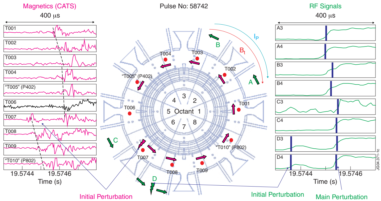
Figure 1: Example of the toroidal propagation of an ELM perturbation seen on magnetic coils and reflected voltages on the antenna transmission lines in JET. Vertical lines on the RF measurements indicate the software evaluated times of reaction. Straps D3 and D4 measure the “initial perturbation” in this case.
