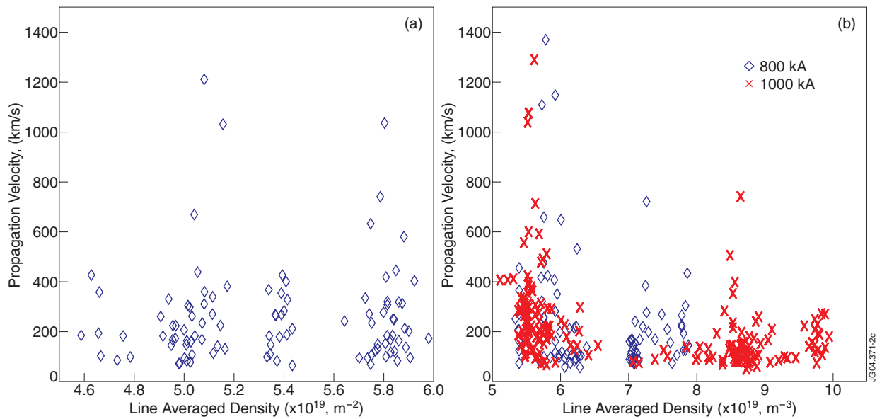
Figure 2: Velocities of propagation of the ELM perturbation as measured by ICRF antennas, depending on central line averaged densities for JET (a) and ASDEX Upgrade (b).
