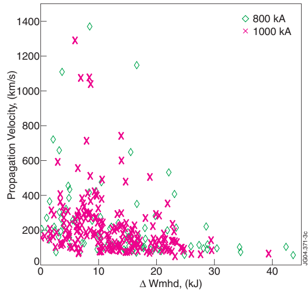
Figure 3: Velocity of propagation of the ELM perturbation vs. change of diamagnetic energy for ASDEX Upgrade.
