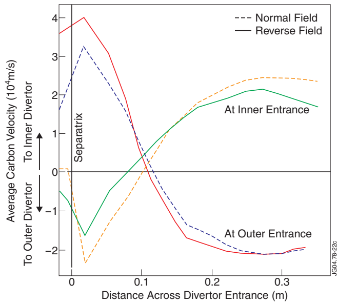
Figure 6. The EDGE2D average carbon velocity was little changed at the inner and outer divertor entrances for cases with only an external deuterium force.
