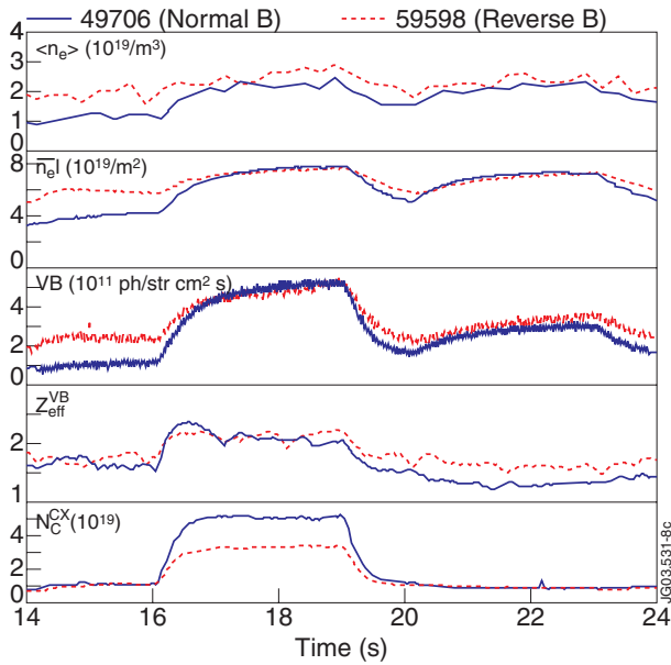
Figure 3. Time evolution of the volume averaged electron density, the line averaged electron density, visible Bremsstrahlung intensity, VB deduced Z_{eff} and the charge exchange deduced total carbon content in the core. The two plasmas are the normal and reverse field plasmas of Figures 1 and 2 and Table I.
