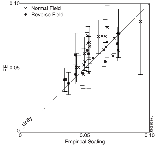
Figure 4. The carbon fuelling efficiency for the reverse field L-Mode plasmas plotted against the normal field empirical scaling [1]. The uncertainty arises primarily from the differencing of the Z_{eff} values (Fig. 3).
