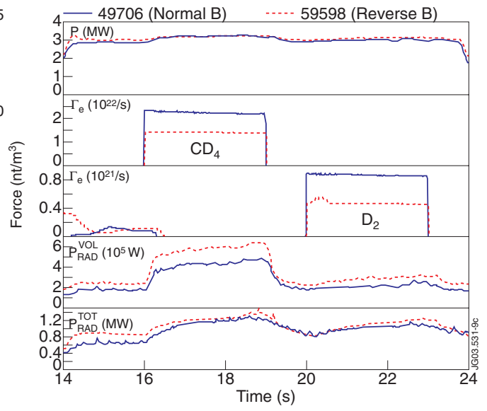
Figure 2. Time evolution of the applied power, the electron injection rates of CD_4 and D_2 , and the power radiated from the core and the total including the X-point region for the cases in Table I and Figure 1.
