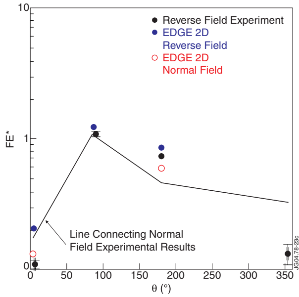
Figure 5. The carbon fuelling efficiency normalized to the mid-plane normal field scaling [1] plotted against the poloidal angle of methane injection. The line connects the normal field experimental results.
