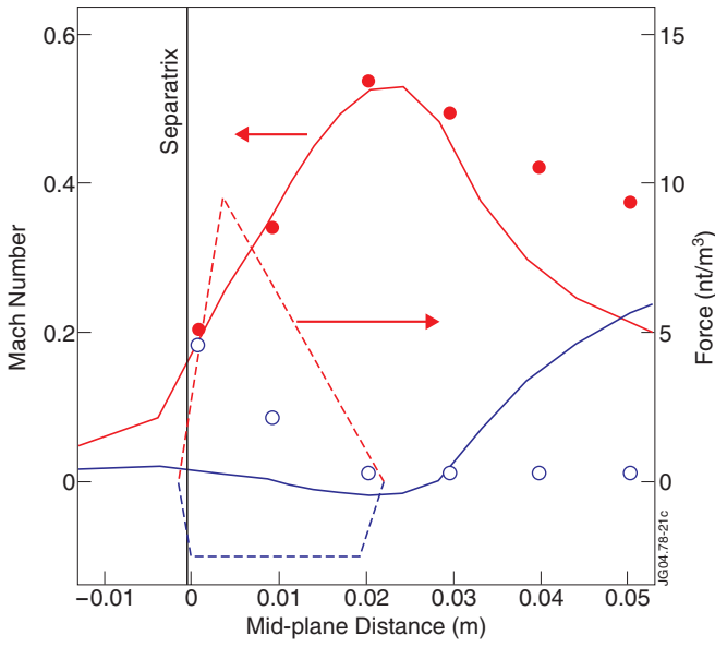
Figure 1. The Mach number simulated by EDGE2D (lines) and average values measured by the JET reciprocating probe [8]. The dashed lines are the external deuterium forces with no force acting on the carbon (Table I).
