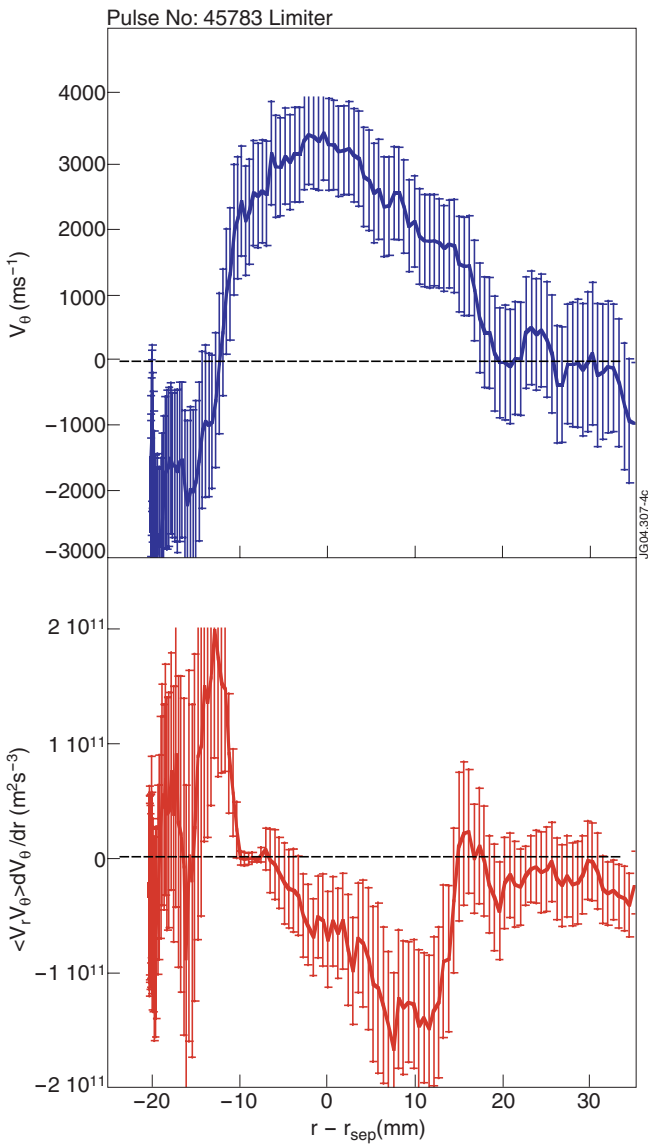
Figure 3: Poloidal velocity of fluctuations and turbulence production term measured in JET plasma Pulse No: 45783 under limiter configuration, ohmic heating.
