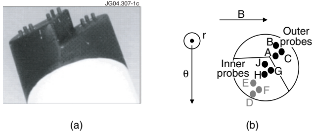
Figure 1: Multiple Langmuir probe used for measurements in JET tokamak (a). Schematic view of probes in the array and orientation with respect to magnetic field (b).
