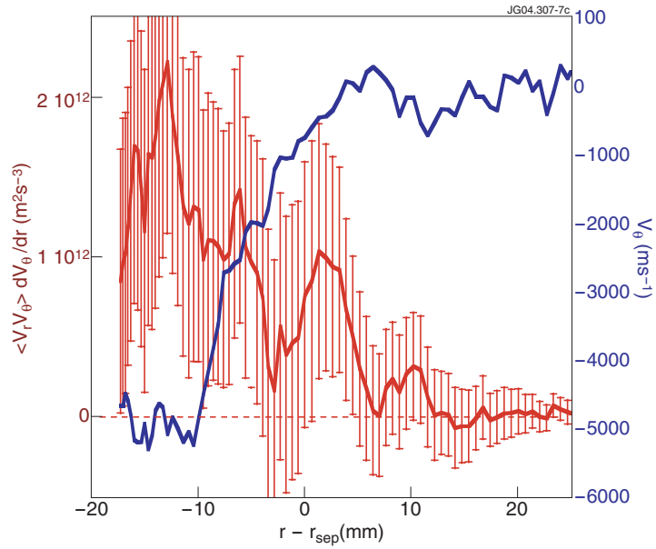
Figure 6: Turbulence production term and poloidal velocity of fluctuations measured in JET plasma Pulse No: 54278 under divertor configuration.
