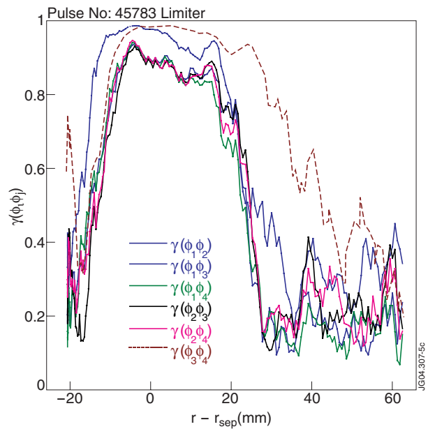
Figure 4: Coherence between potential signals measured in JET Pulse No: 45783 under limiter configuration, ohmic heating.
