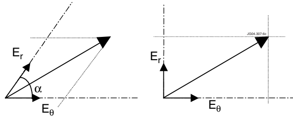
Figure 5: Schematic view of the electric field measurement in a orthogonal and non-orthogonal axis frame of reference ( \alpha \approx 60^\circ ).
