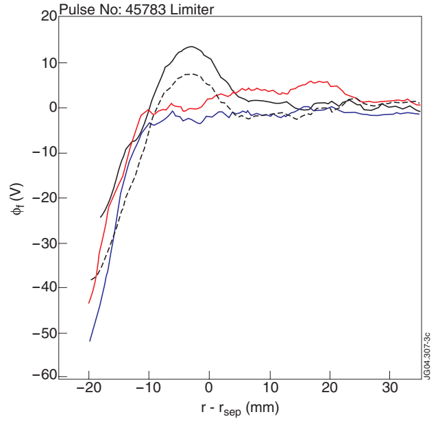
Figure 2: Profile of floating potential measured by the Langmuir probe in a limiter discharge (Pulse No: 45783).
