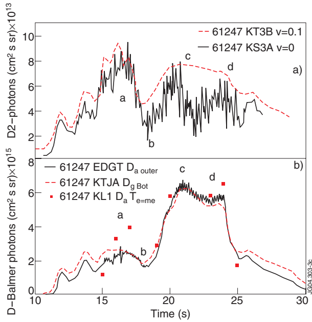
Figure 3: Behaviour of the molecular (a) and atomic (b) deuterium intensities integrated over the outer divertor region during a sweep of the separatrix from the horizontal to the outer vertical target plate in L-mode (JET Pulse No: 61247) a) full line: KS3A v=0 , dashed line: KT3B v=0-1 b) full line: D_{\alpha} -filter system, dashed line: D_{\gamma} from KT3A, points: D_{\alpha} -camera KL1.
