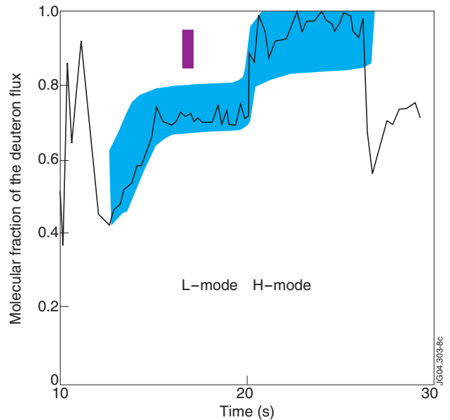
Figure 8: Ratio of protons from molecules to the total (proton) influx during JET Pulse No: 61248 in the outer divertor. The shadowed area describes the variation introduced by the inaccuracies of S/XB - and D/XB -values. The rectangle is from EDGE2D/NIMBUS calculations.
