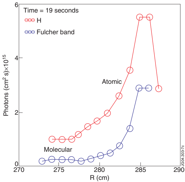
Figure 7: radial distribution of the atomic D_{\gamma} -line and the Fulcher- \alpha emission from deuterium molecules
