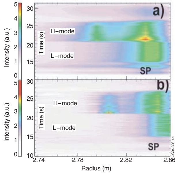
Figure 4: Atomic (a: D_{\gamma} ) and molecular (b: v=0-1 ) intensity distributions over the horizontal target plate during the L- and H-mode for JET Pulse No: 61248 from KT3A,B.
