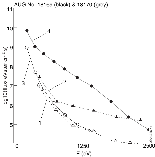
Figure 4: Hydrogen (dashed lines 1, 2) and Deuterium (solid lines 3, 4) atom spectra observed with NPA in the similar AUG ICRF discharges ( P_{RF} \approx 370\text{ kW} , p_{He} \approx 4.0 \times 10^{-2}\text{ Pa} ) at B_T = 2.0\text{ T} (black) and B_T = 1.0\text{ T} (grey).
