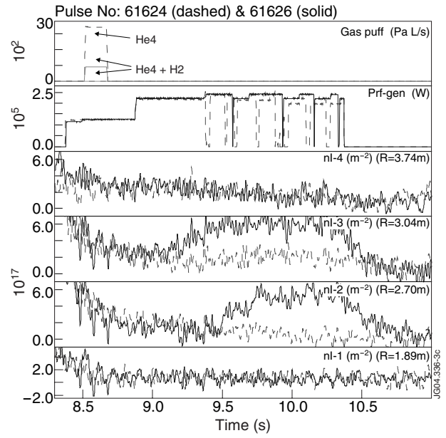
Figure 3: Evolution of the line-integrated density for two similar ICRF discharges in JET performed in helium (Pulse No: 61624, dashed) and in a gas mixture of \sim 80\%He and \sim 20\%H_2 , (Pulse No: 61626, solid).
