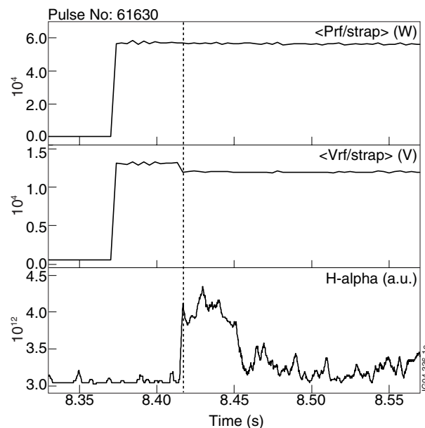
Figure 1: The transition from the neutral gas breakdown phase to the ICRF discharge phase in JET.
