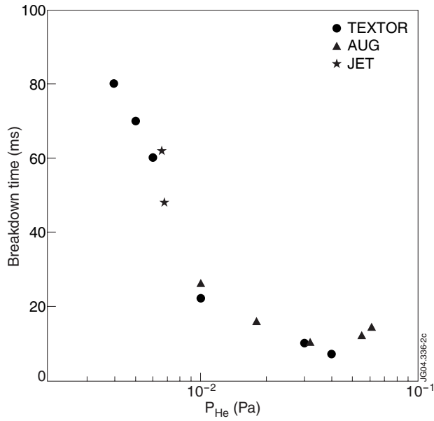
Figure 2: Pressure dependence of the RF breakdown time derived from the H_{\alpha} emission analysis ( P_{RF}/\text{antenna strap} \approx 30\text{-}50\text{ kW} , f \approx 30\text{ MHz} , \omega = 4\omega_{cHe+} = 2\omega_{cD} = \omega_{cH} ).
