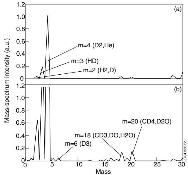
Figure 5: Mass-spectrum of the residual gas in the JET vessel before (a) and after (b) the ICRF conditioning Pulse No: 61631 (constant P_{RF-gen} \approx 230\text{ kW} , decayed B_T = 2.45\text{-}1.85\text{ T} and p_{tot} \approx (7\text{-}1) \times 10^{-3}\text{ Pa} ).
