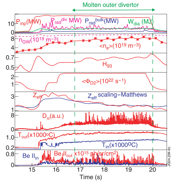
Figure 5. Plasma parameters obtained during a high power JET divertor discharge on the Be Mk I divertor in which the outer divertor target surface reached the Be melting temperature during more than 3 secs. Large Be influxes were measured at every ELM by the Be II line emission from the outer divertor.
