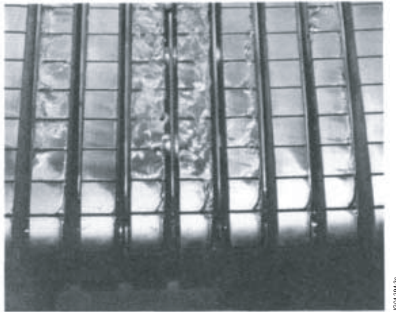
Figure 2. Photograph of a section of the JET beryllium belt limiter showing heavy melting and melt layer displacement following high power limiter experiments at JET.
