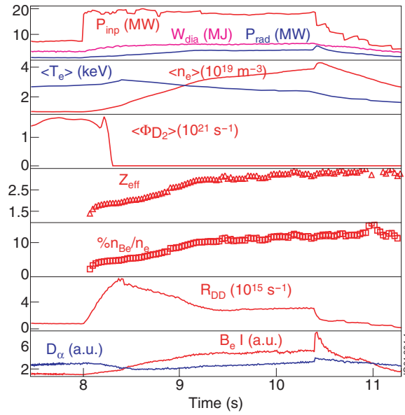
Figure 3. Plasma parameters obtained during a high power JET beryllium limiter discharge, in which a beryllium droplet is seen to fall into the plasma from the top upper limiter at the time marked by the vertical line.
