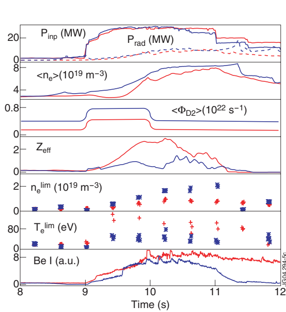
Figure 4. Plasma parameters obtained during two high power JET beryllium limiter discharges with (blue traces) and without (red traces) strong gas fuelling. For the discharge with strong gas fuelling the Z_{\text{eff}} remains low for the whole duration of the high power phase.
