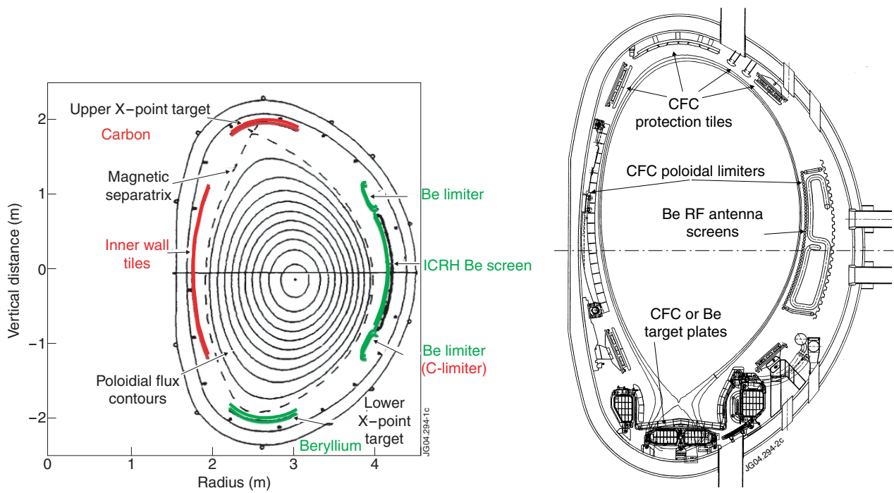
Figure 1. a) JET plasma facing components (divertor targets, belt limiters and ICRH screens) for the operation period 1990-1991 and 1991-1992. In the period 1991-1992 the lower toroidal belt limiter was replaced by a carbon limiter. b) JET plasma facing components (divertor target, poloidal limiters and ICRH screens) for the operation period 1994-1996, in which two materials were tested for the divertor target tiles C and Be.
