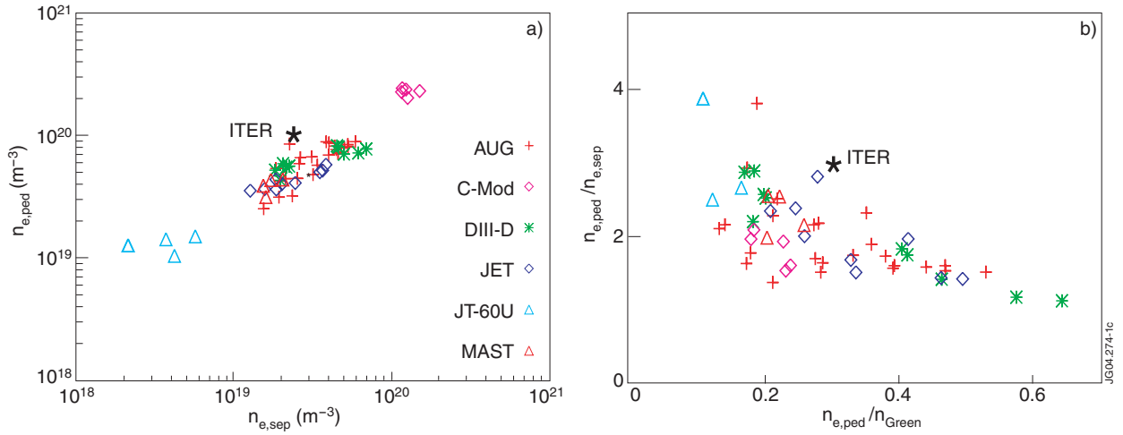
Figure 1: a) Pedestal density versus separatrix density and b) n_{e,ped}/n_{e,sep} versus n_{e,sep} normalised by the Greenwald density. The data base comprises 28 type-I ELMy H-mode phases from AUG, 10 from DIII-D, 9 from JET, 4 from JT-60U, 1 ELMy and 4 EDA H-modes from C-Mod and 4 ELMY discharges with mixed type-I, III characteristics from MAST high-field side measurements. The ITER operating point assumes a pedestal density of 10.5 and a separatrix density of 3.5 \cdot 10^{19} m^{-3} [9].
