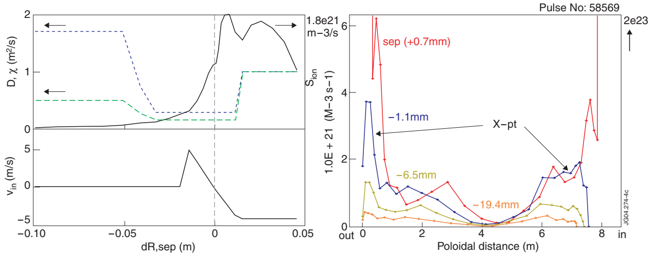
Figure 4: Radial (outer midplane) and poloidal profiles of the neutral ionisation rate from EDGE2D calculations of a JET ELMy H-mode discharge. The transport coefficients are also shown to indicate the ETB position. The poloidal distribution shown on the rhs shows a high neutral source rate around the X-point outside the separatrix, which decays very fast towards the core.
