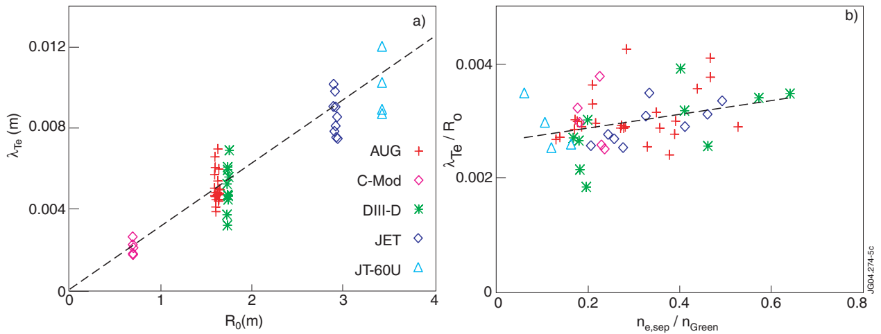
Figure 5: a) midplane temperature e-folding length versus major machine radius R_0 . The dashed line shows \lambda_{Te} = 3.1 \cdot 10^{-3} R_0 obtained from fitting. b) \lambda_{Te} normalised by machine size versus normalised separatrix density.
