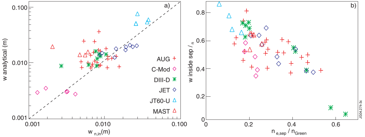
Figure 3: a) Measured density width versus neutral penetration depth from the analytical model. b) Steep density region inside the separatrix divided by full width derived from tanh analysis versus normalised separatrix density. An outward shift of the density profile is observed with increasing Greenwald fraction of the separatrix density.
