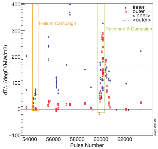
Figure 2: \Delta T/P_{cond} for inner and outer targets over a period of 3 years operation. Dashed lines indicated the average value excluding operation in reversed B or He. The average values correspond to \alpha_{inner} = 6\text{ kW/m}^2/\text{K} , and \alpha_{outer} = 200\text{ kW/m}^2/\text{K} .
