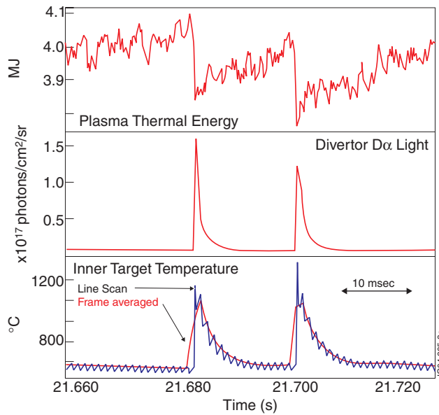
Figure 3: The temperature evolution at the inner target for ELMy H-mode plasma (Pulse No: 55936). The jitter with \sim 1.3\text{ msec} period is an artefact of the IR measurement which scans an image line by line at a rate 1.3\text{ msec/frame} .
