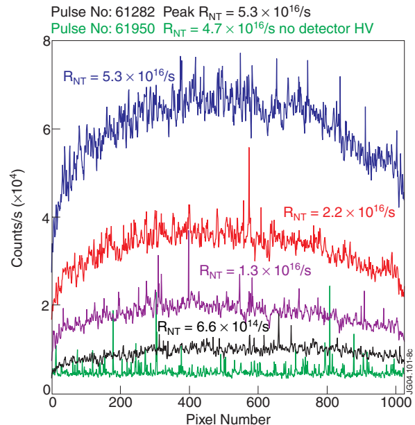
Figure 8. Increase in SOXMOS detector background with neutron yield. The lowest trace has no detector high voltage applied and shows the noise level in the diode array alone
