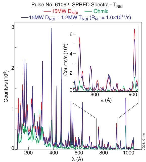
Figure 4. SPRED spectra from T beam injection pulse showing no increase in background noise even at the time of the peak neutron rate (which was the highest for TTE)
