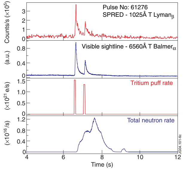
Figure 6. Spectroscopic monitoring of tritium gas injection by both visible and VUV instruments – in this case a double T puff.
