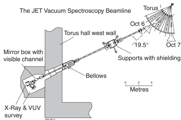
Figure 1. Location of JET VUV survey spectrometer (SPRED). The bunker is shared with a Bragg rotor X-ray spectrometer and a visible channel.
