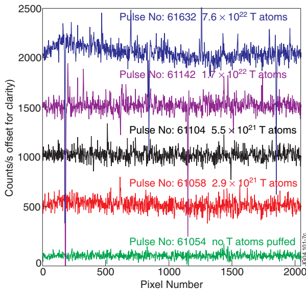
Figure 7. Progression of tritium retention in the SPRED detector. Data from successive Dry Runs is shown. Total T atoms puffed prior to each pulse are indicated. Pulse 61632 is after TTE had concluded
