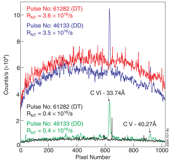
Figure 9. Effect of 2.5 MeV DD neutrons (Torus valve open) and 14 MeV DT neutrons (Torus valve closed) on the SOXMOS background levels for equivalent total neutron rates.
