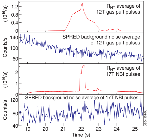
Figure 5. SPRED background noise levels during tritium gas puffing and beam injection with instrument valved off from the torus.
