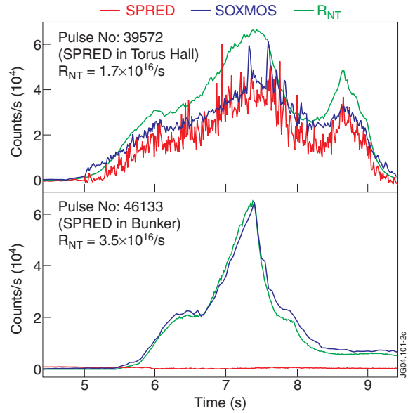
Figure 2. Background noise reduction in SPRED after relocation to bunker. Peak R_{NT} values are quoted.
