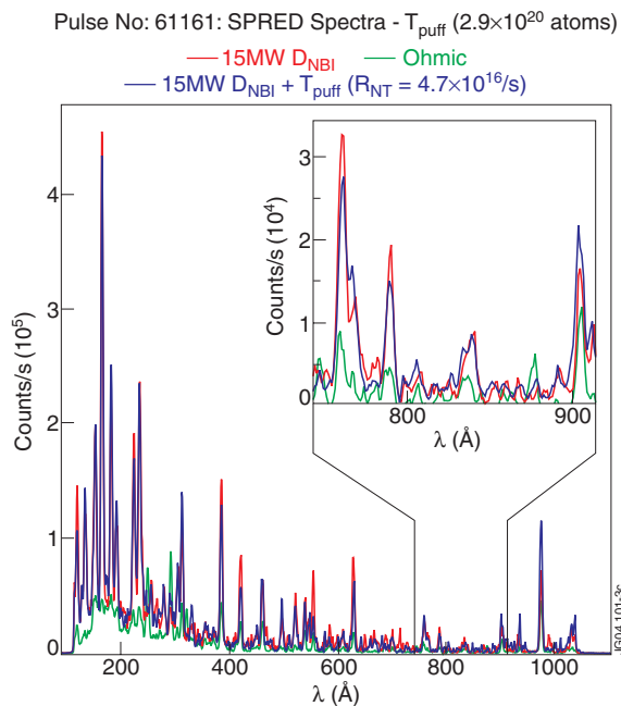
Figure 3. SPRED spectra from T puff pulse showing no increase in background noise even at the time of the peak neutron rate.
