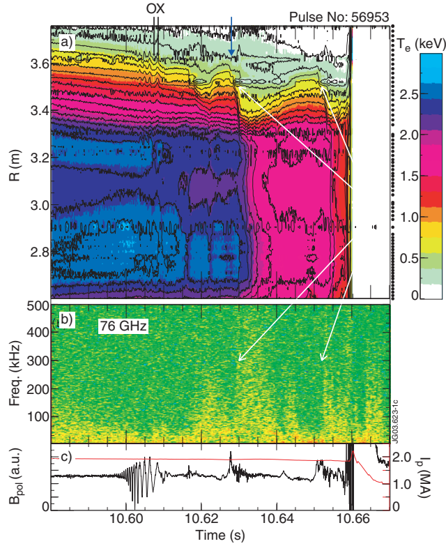
Figure 1: Synchronized time evolution of some plasma parameters during disruption. (a) T_e measured with ECE radiometry. Dots at right indicate channels positions. (b) Spectrogram of fluctuations from 76GHz X mode LFS reflectometer channel. The blue arrow in (a) indicates position of cut-off layer. White arrows indicate clear correlations between variations in the signals of the radiometer and the reflectometer. (c) Perturbed poloidal magnetic field measured inside the vessel at the LFS and plasma current.
