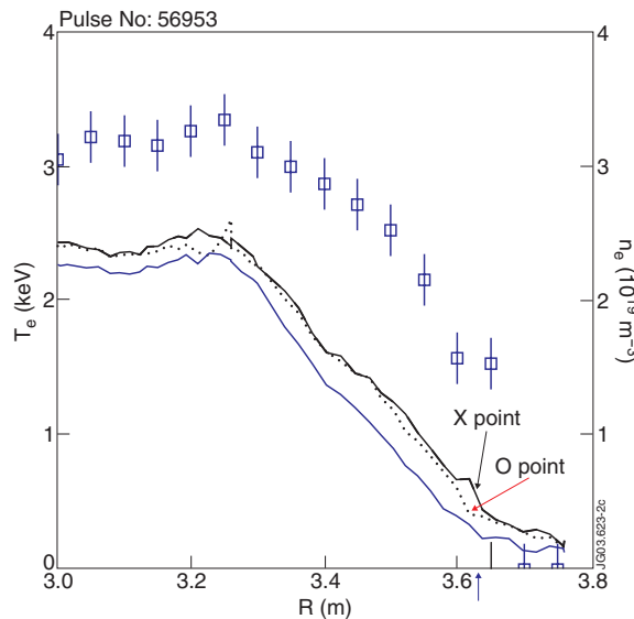
Figure 2: T_e ECE profiles (lines) and n LIDAR profile (squares). Profiles in blue were measured at 50.6276 s. In red and black at 10.6074s and 10.6085s respectively (see black arrows in Fig.1(a)). The red and black T_e profiles are shown to indicate the radius of the m/n = 2/1 island. Just like in Fig.1(a) the blue arrow indicates the position of the 76 GHz cut-off layer.
