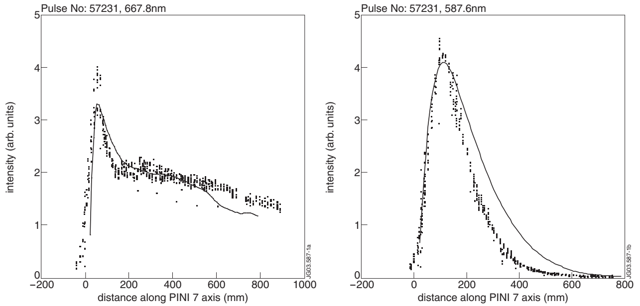
Figure 1: Measured (dots) and modelled (line) HeI beam emission profiles of JET Pulse No: 57231, plotted along the axis of the injected helium beam. (helium doped PINI 7)
