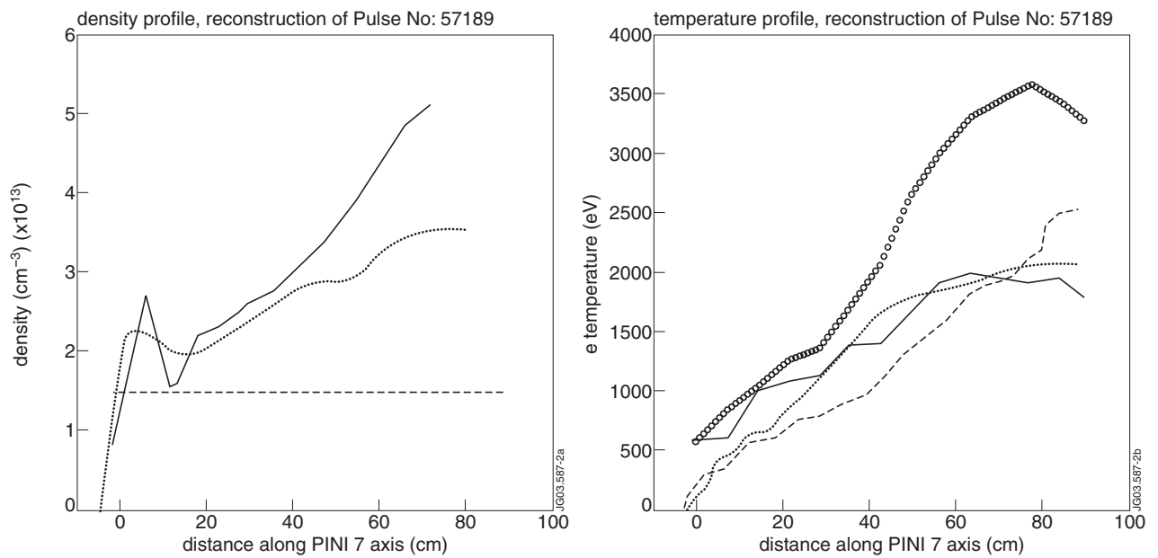
Figure 2: Plasma density- and temperature reconstruction for JET Pulse No: 57189, plotted along the axis of the injected helium beam. (He doped PINI 7) Full curve in both graphs: reconstructed profiles dotted curves in both graphs: core- and edge lidar density and temperature profiles dashed curve in right graph: ECE temperature profile small dots in left graph (flat line): starting situation for density reconstruction open circles in right graph: starting situation for temperature reconstruction.
