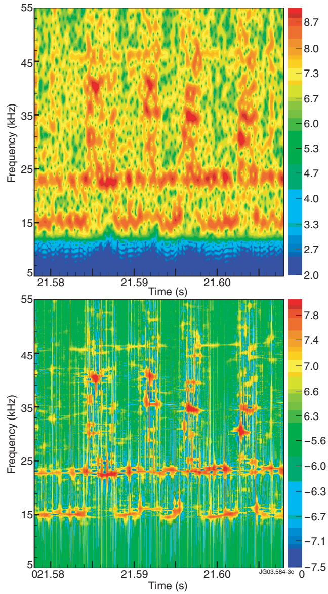
Figure 3: Analysis of a magnetic pick-up coil signal (JET Pulse No: 55976), using (a) the spectrogram with l = 255 , and (b) the Choi-Williams distribution with l_{\tau} = 2047 , l_{\mu} = 255 and \sigma = 0.5 . The interruption of the WB modes by the type-I ELM precursor is best seen with the Choi-Williams distribution.
