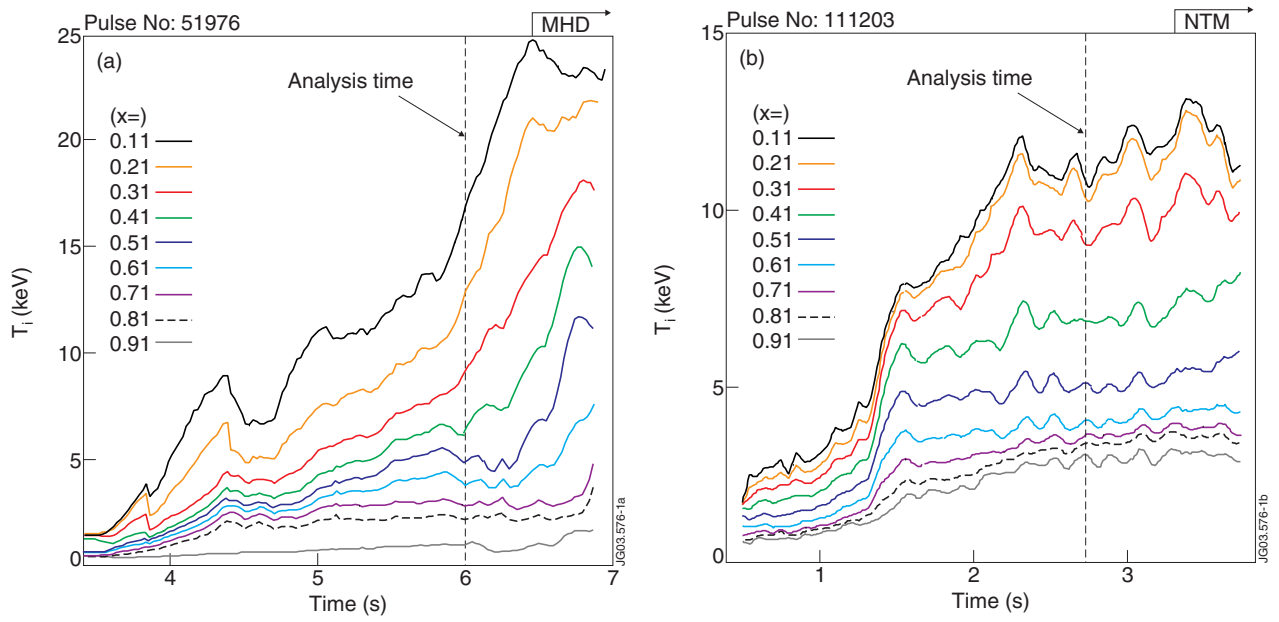
Figure 1: Time evolutions of ion temperatures in the a) JET and b) DIII-D plasmas
