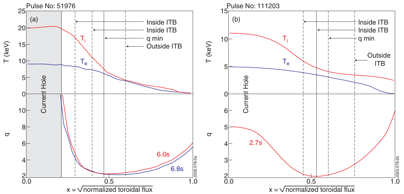
Figure 2: Measured profiles of temperatures and q in a) JET and b) DIII-D plasmas
