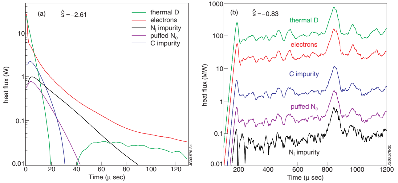
Figure 3: Nonlinear GS2 results for heat flux in the JET plasma at a) x=0.3 , and b) x=0.4
