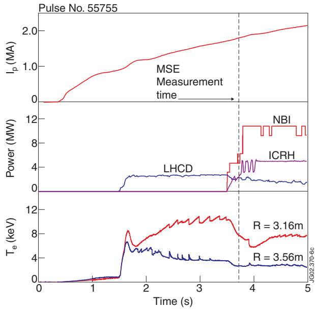
Figure 1: Current hole discharge parameters.
