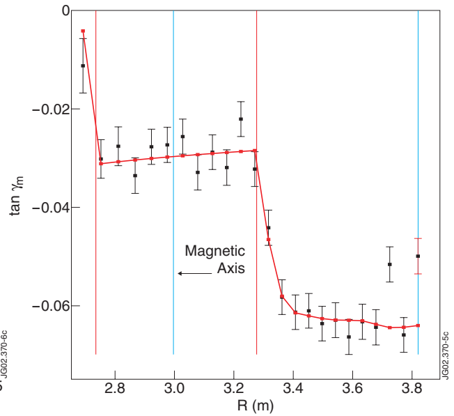
Figure 2: MSE pitch angle profile (points) and ESC reconstruction best fit (solid line).
