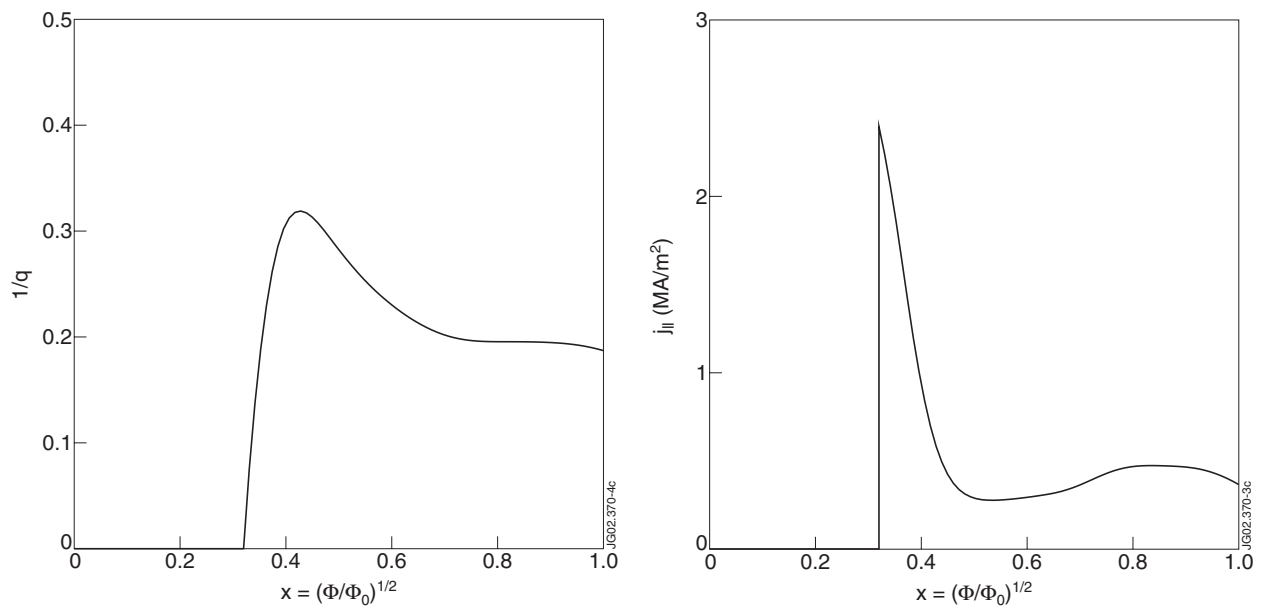
Figure 3: \tau = 1/q profile (left) and j_{\parallel} profile (right) from ESC reconstruction of current hole discharge shown in figures 1 and 2.
