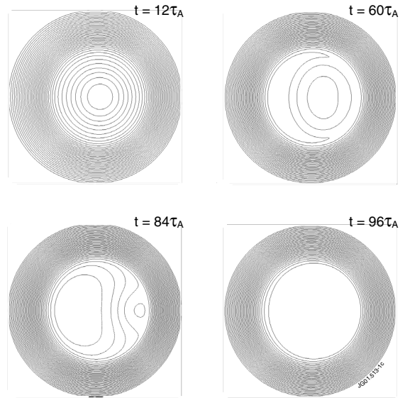
Figure 5: Poloidal flux map, \psi(R, Z) , at four times in axisymmetric sawtooth period from M3D simulation with circular plasma cross section.
