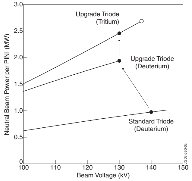
Figure 6. Estimated neutral beam power injected to JET plasma from a single Octant 8 PINI.
