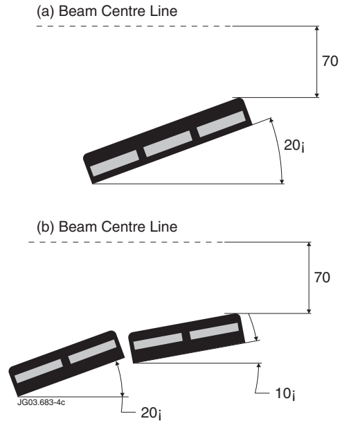
Figure 4: Modification of the Box Scraper geometry: (a) old configuration and (b) new configuration.
