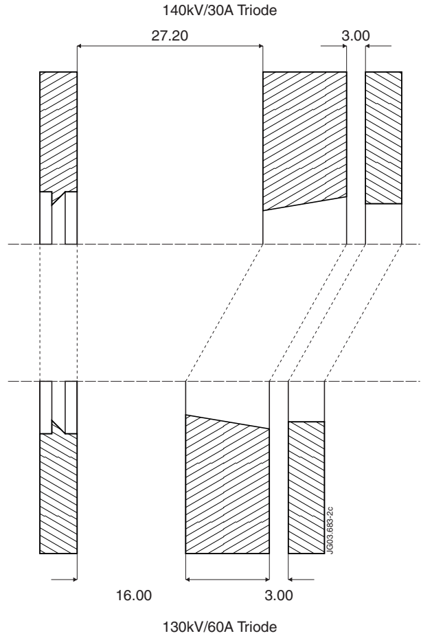
Figure 2. Modification of the JET triode PINI accelerator geometry.
