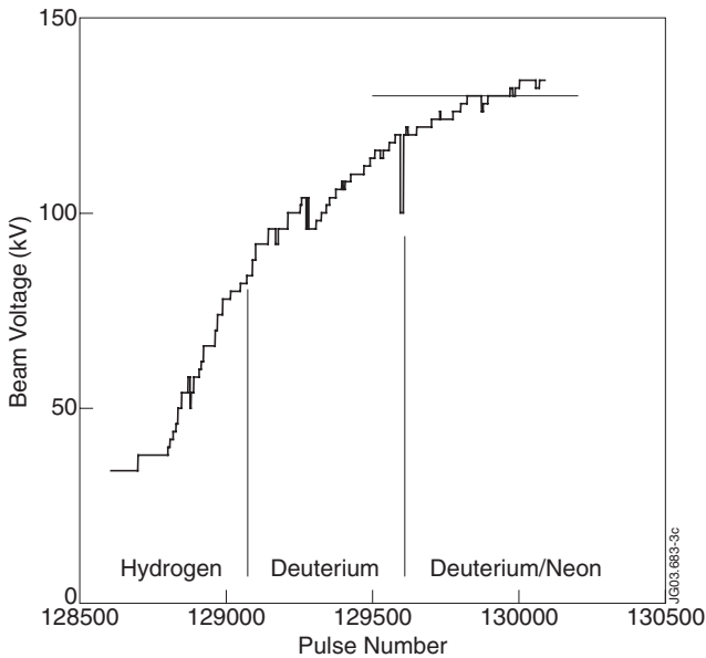
Figure 3: Conditioning history of upgraded triode PINI. Deuterium/neon mix is used to allow conditioning above maximum voltage while maintaining beam current below the power supply limit of 60A.
