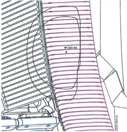
Figure 5. Shine-through power density contours ( 1 \text{ MW/m}^2 and 0.5 \text{ MW/m}^2 ) under conditions of minimum beam attenuation (i.e. minimum plasma density) overlaid on the outer wall of the JET machine (ICRH antenna.).
